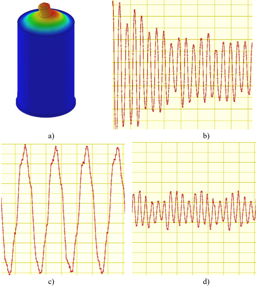
Fig. 5.4. Outer cap with accelerometer and vibration acceleration in axial direction (a): b) free oscillations after impact, frequency – 465 Hz; c) forced oscillations on the EMC housing; operating frequency – 100 Hz; d) forced oscillations on the input window. Scale at y axis: 0.05 g/div, at x axis: 5 ms/div
