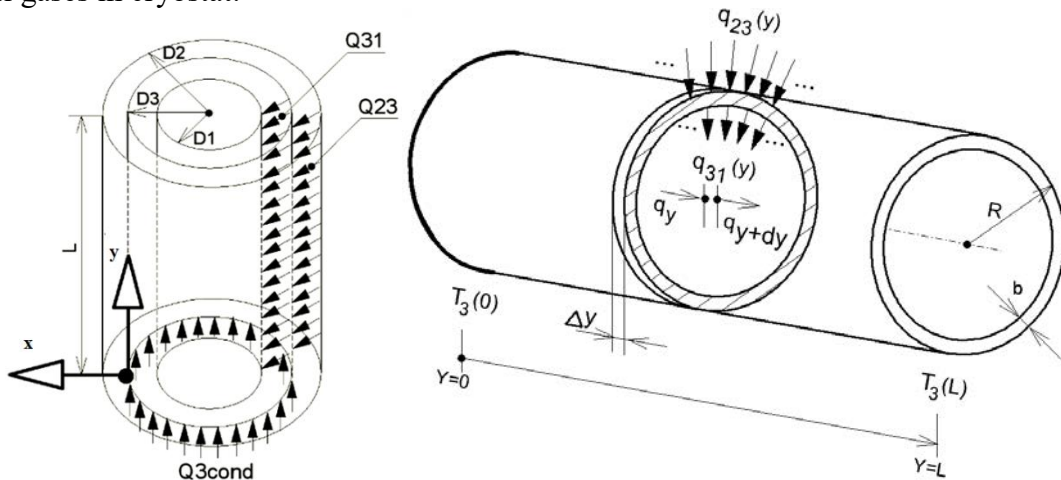
Fig. 4.5. Heat shield calculation model in cryostat (left); energy balance for infinitely small element (right).
