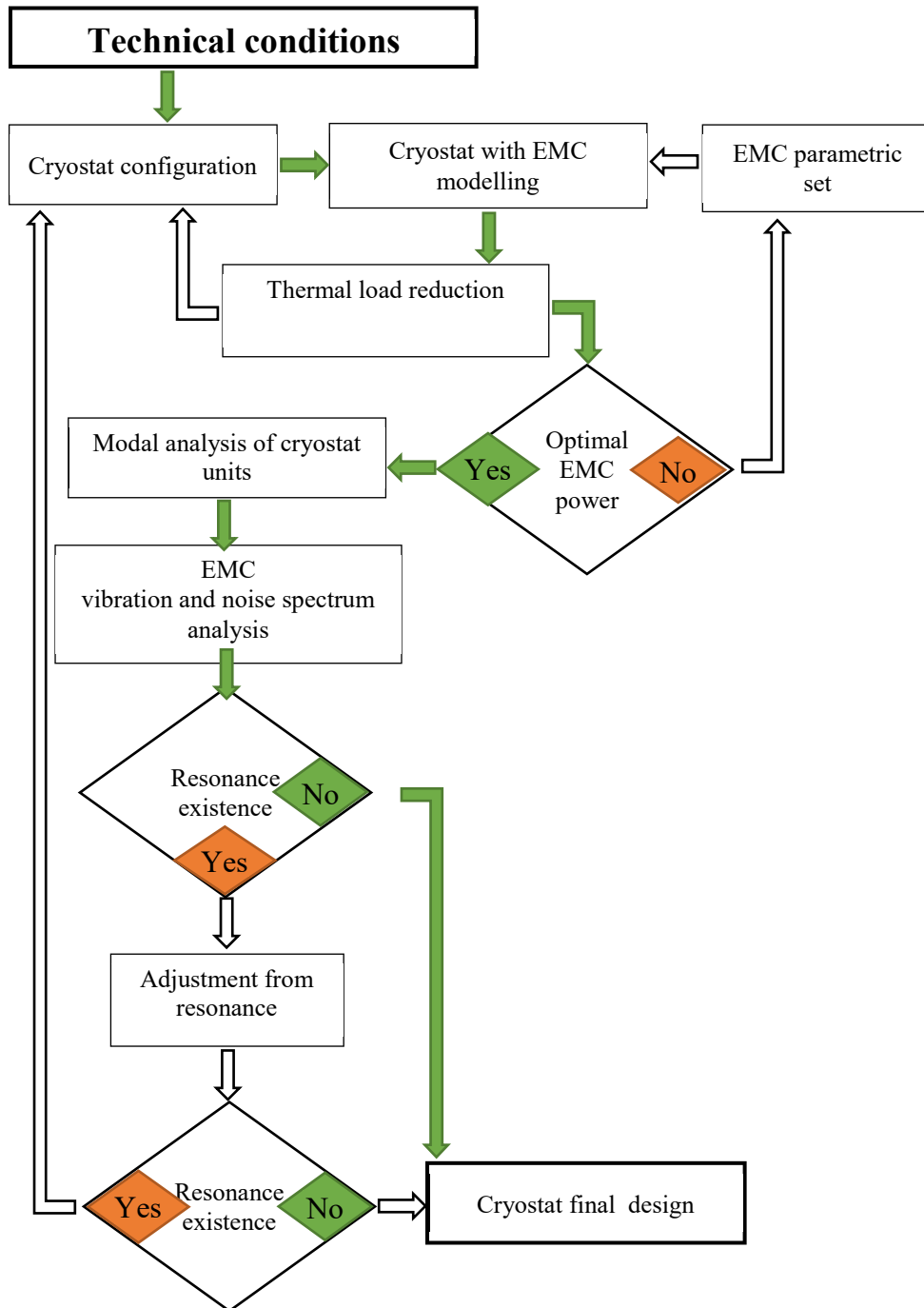
Fig. 3.1. Structure of complex approach for the design of gamma spectrometers cryostats with EMC.
