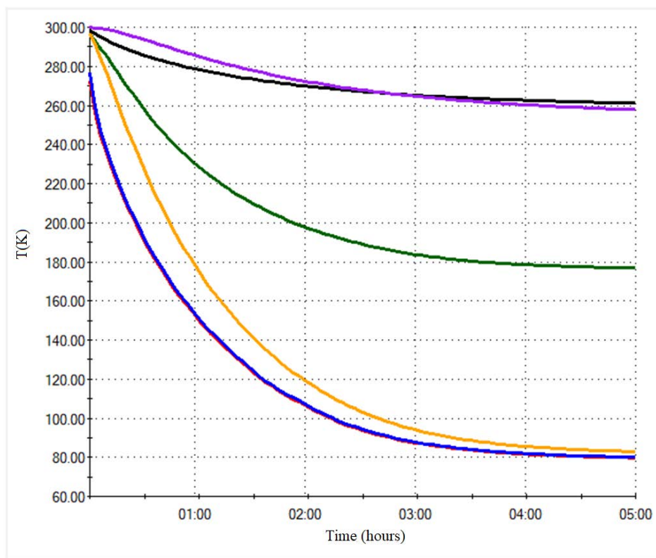
Fig. 4.9. Cooling curves for cryostat (Fig. 4.8.) components.
