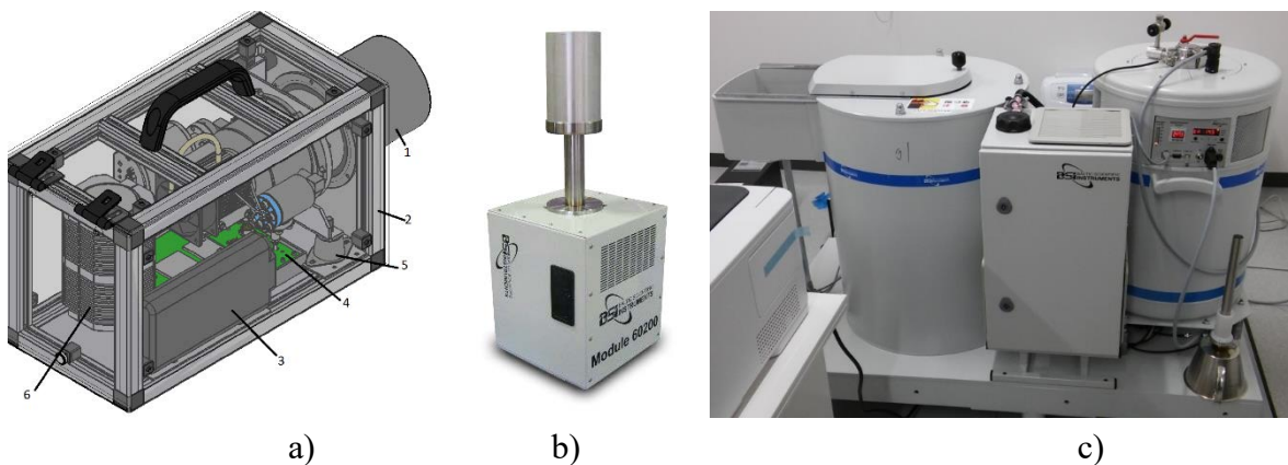
Fig. 6.1. a) portable gamma spectrometer HandSPEC ; b) Monolith laboratory gamma spectrometer; c) Nicole gamma spectrometer with hybrid cooling.
