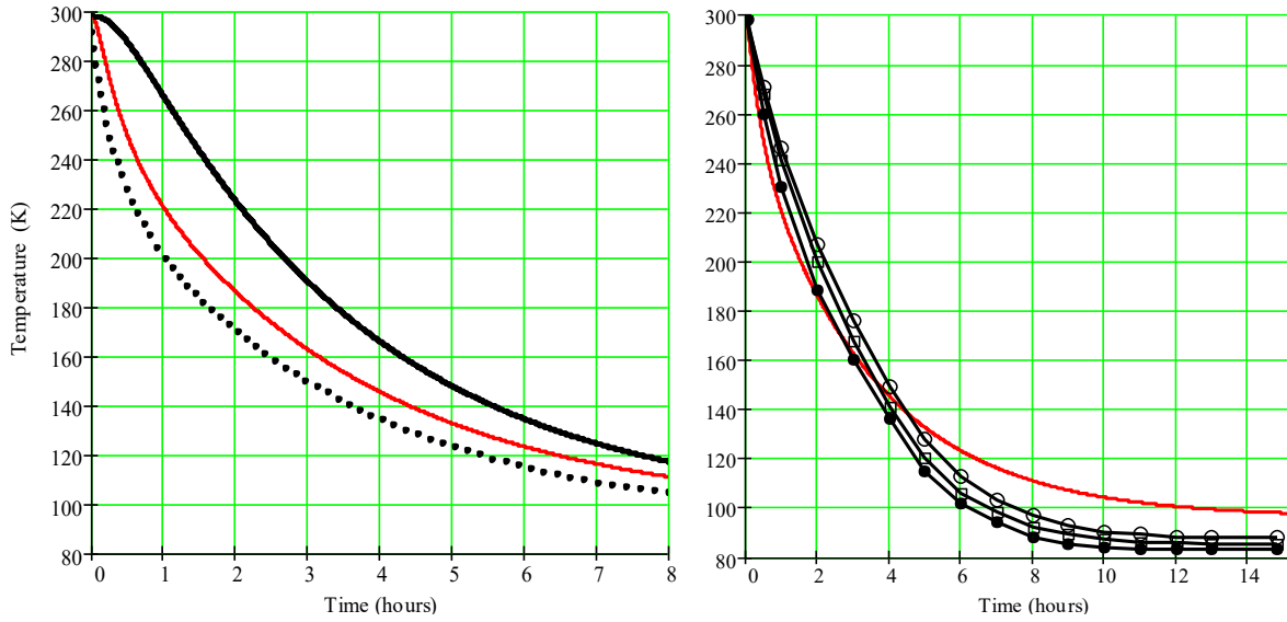
Fig. 4.4. Detector (black curve), detector holder (red curve), sorbent tank (dotted line) calculated cooling curves (left side); experimental (black curves) and calculated (red curves), comparison (right side).
