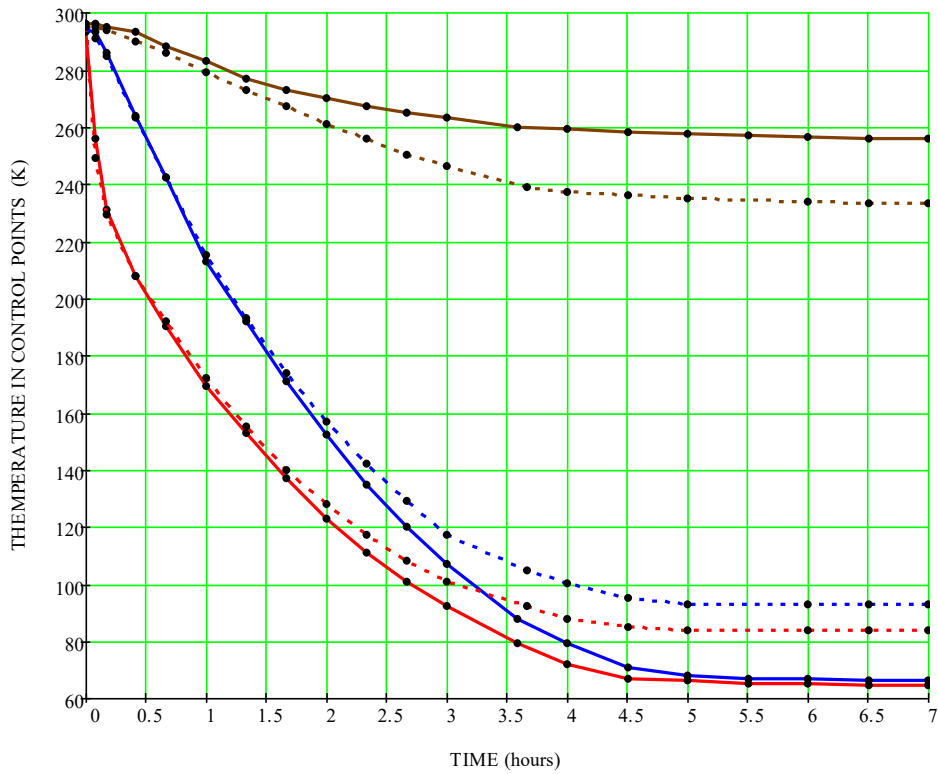
Fig. 4.10. Cryostat with thermal shield cooling curves (continuous lines: p < 10^{-5} mbar; dotted line: p = 4 \cdot 10^{-3} mbar). Red curves – temperature at the cold end of EMC; blue curve – temperature on HPGe detector holder; brown curve – temperature on the thermal shield.
