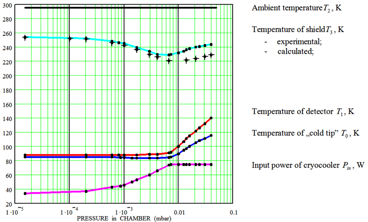
Fig. 4.11. Changing the temperature at the control points and changing the EMC input power at different pressures in a cryostat vacuum chamber.
