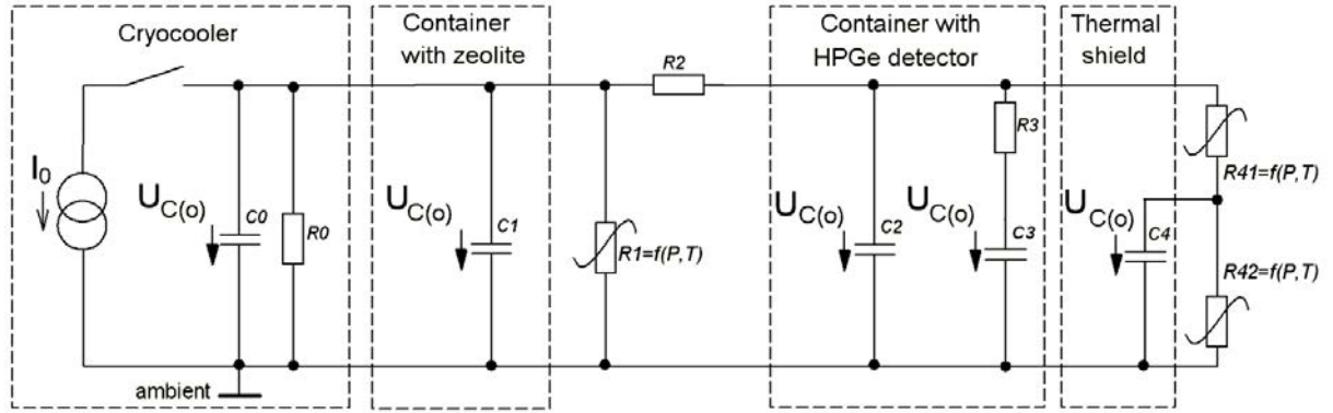
Fig. 4.2. Equivalent thermoelectric model for cryostat with EMC and thermal shield for cooling process analysis.
