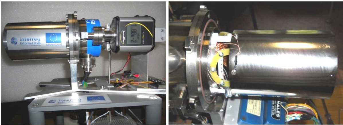
Fig. 4.6. Overview of cryostat for studies (left) and thermal shield in assembled form (right).
