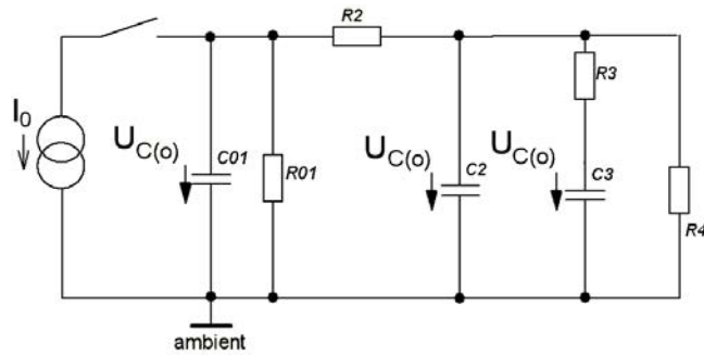
Fig. 4.3. Linearized equivalent cryostat with EMC model.
