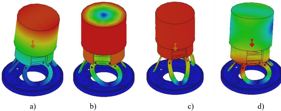
Fig. 5.2. Lower modes of detector unit: a) and d) bending; b) torsional; c) axial.
