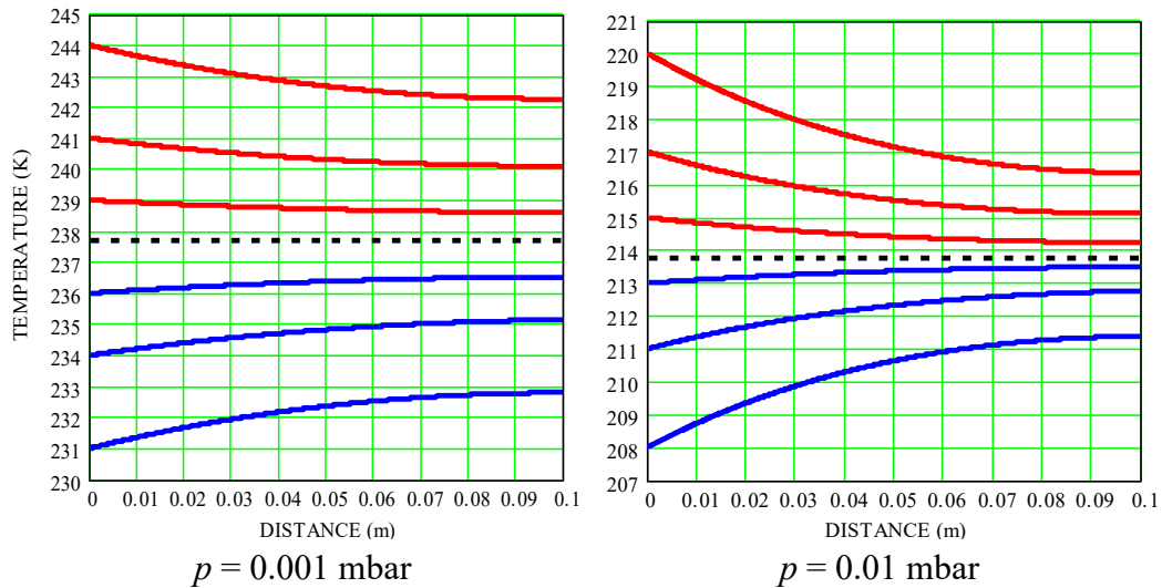
Fig. 4.7. Distribution of temperature on the surface of stainless-steel heat shield (0.5 mm thick) for various initial gas temperatures and pressures.
