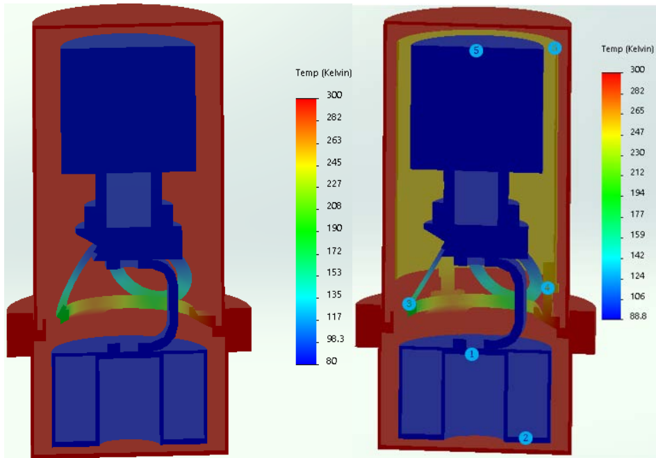
Fig. 4.8. The cryostat temperatures (without the thermal shield (left) and with the thermal shield (right)) have stabilized in the cooling state of Solidworks .
