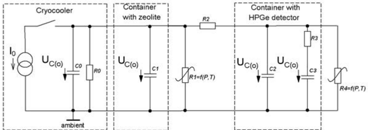
Fig. 4.1. Equivalent thermoelectric model of cryostat with EMC for cooling process analysis.
