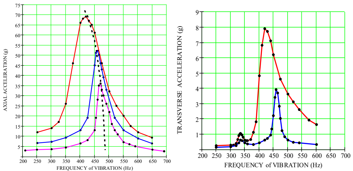
Fig. 5.3. Dependency of the vibration acceleration of the detector unit in the axial (vertical) (left) and transverse (horizontal) (right) direction of the frequency if there is a constant amplitude of the base vibration acceleration: 9g – red line; 4g – blue line; 2g – pink line.
