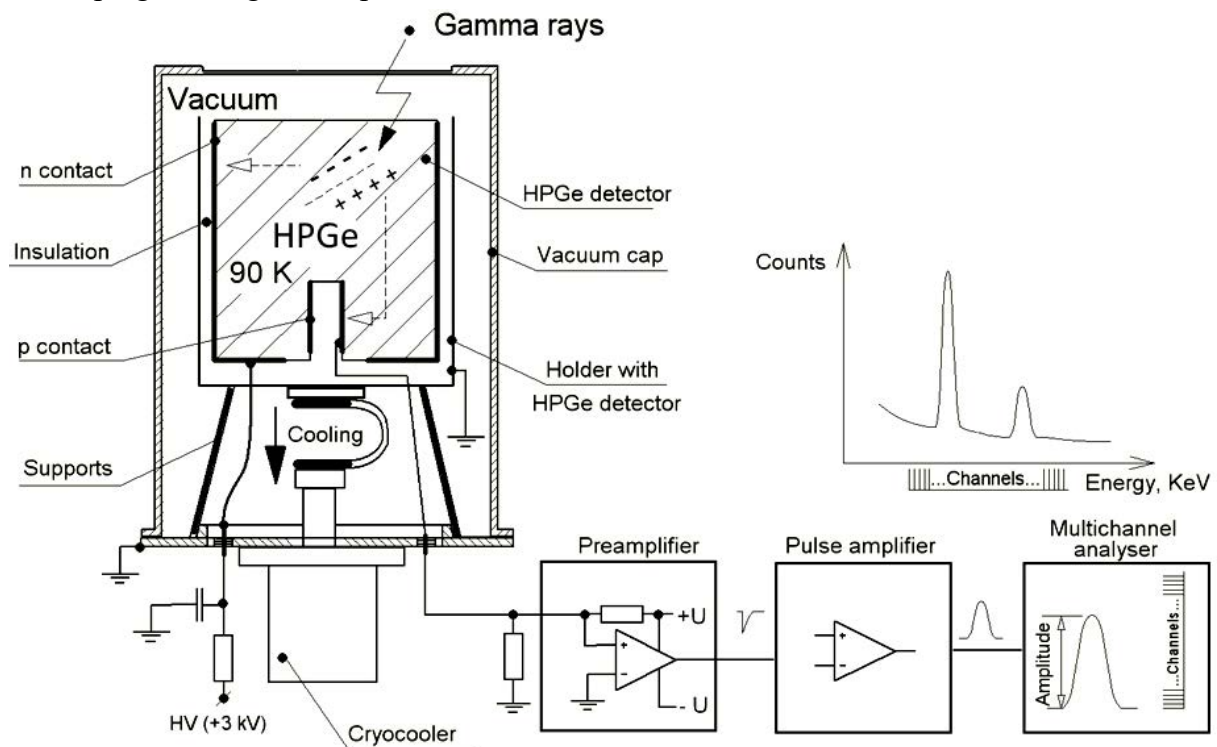
Fig. 1.1. Gamma spectrometer structure based on HPGe detectors.
