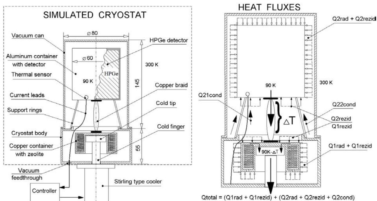
Fig. 2.1. Heat fluxes components in cryostat.
