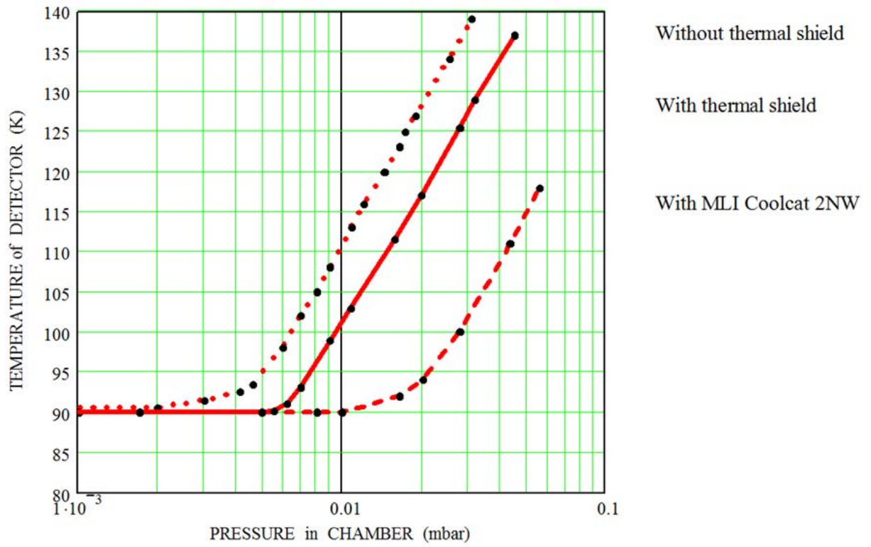
Fig. 4.12. The temperatures of detector for varied pressures in a vacuum chamber without thermal shield (dotted curve); with thermal shield (solid curve) and with MLI (dashed curve).
