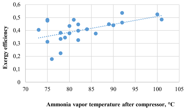
Fig. 2.30. Exergy efficiency of two-stage compressor refrigeration system depending on ammonia vapor temperature after compressor.
