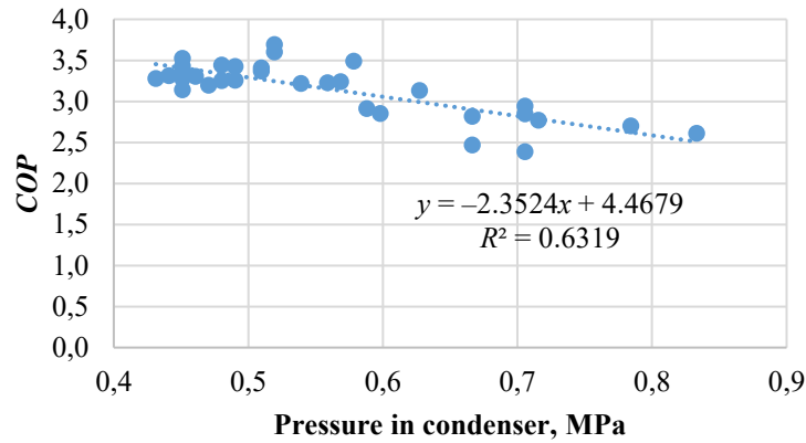
Fig. 2.22. Two-stage compressor COP depending on condenser pressure.
