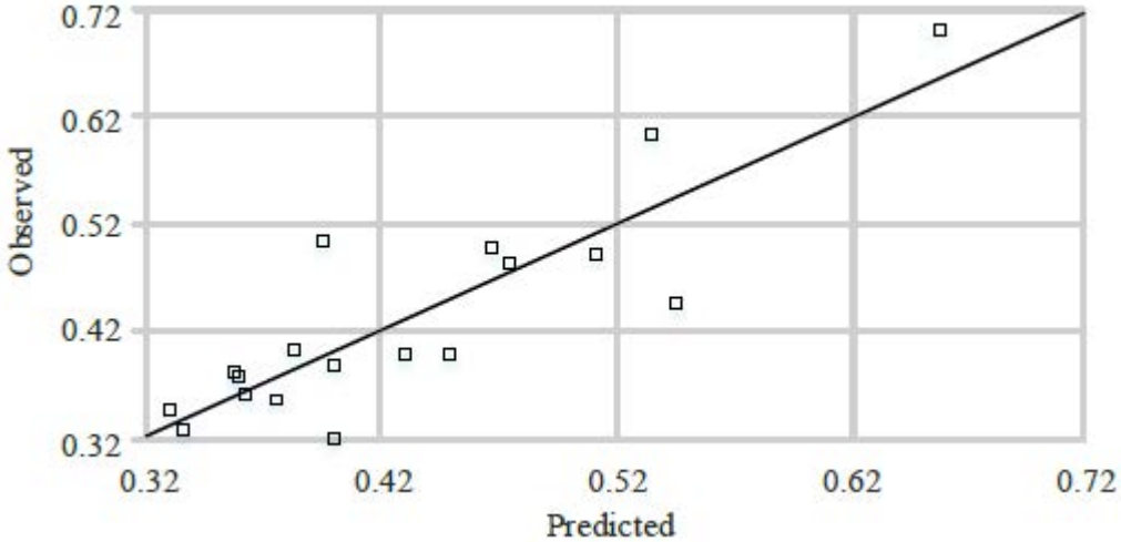
Fig. 2.20. Plot of specific electricity consumption (MWh el /t of net production) – predicted versus observed values.
