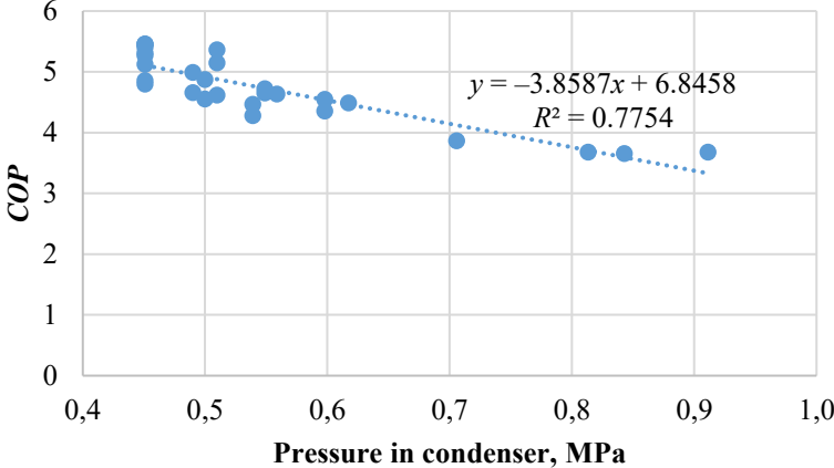
Fig. 2.24. Single-stage compressor COP depending on condenser pressure.
