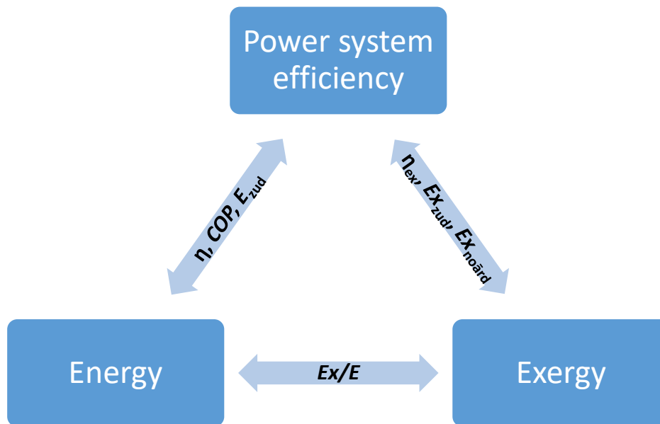
Fig. 1.1. Interaction between power system efficiency and its indicators “energy” and “exergy”.
