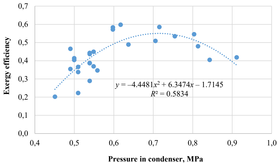
Fig. 2.28. Exergy efficiency of a single-stage compressor refrigeration system depending on the pressure in condenser.
