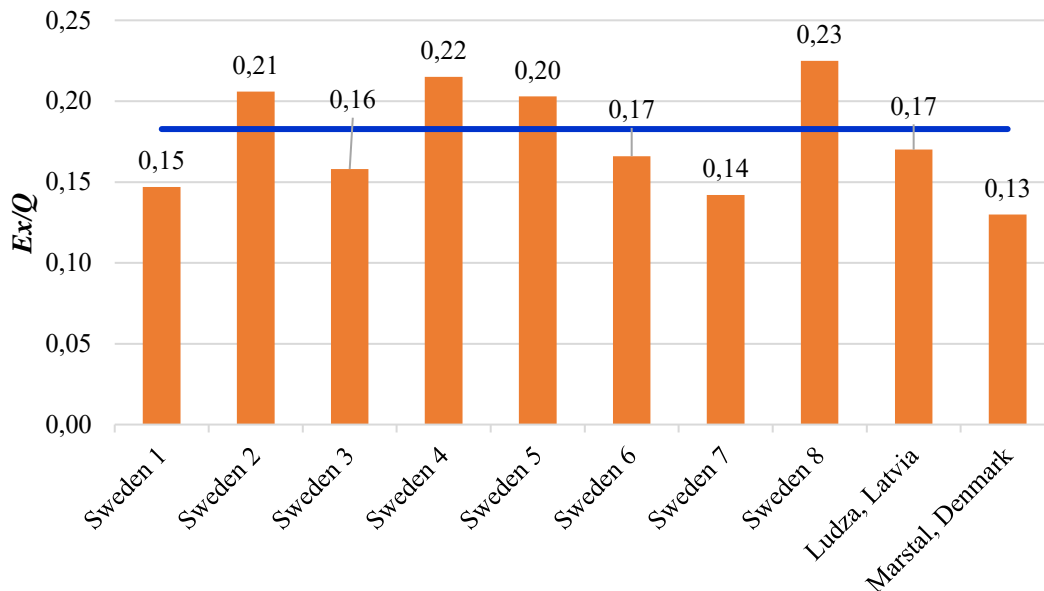
Fig. 2.3. Comparison of exergy factors [6].
