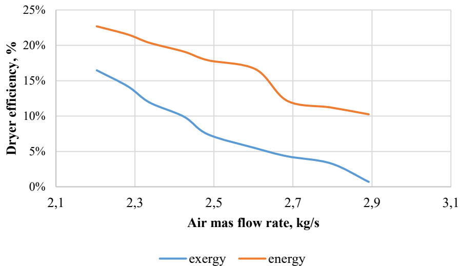
Fig. 2.11. Dryer efficiency versus the flow rate of drying air mass.
