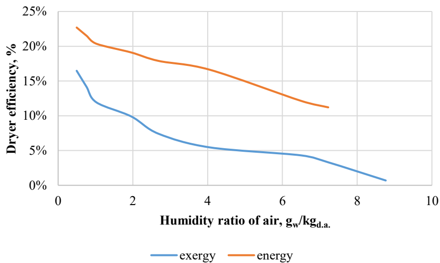
Fig. 2.12. Dryer efficiency versus humidity ratio of drying air.
