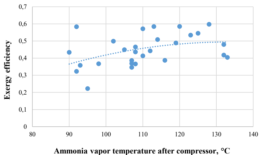
Fig. 2.27. Exergy efficiency of a single-stage compressor refrigeration system depending on ammonia vapor temperature after compressor.
