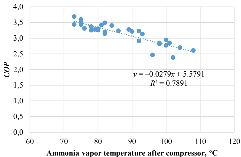
Fig. 2.23. Two-stage compressor COP depending on ammonia vapor temperature after compressor.
