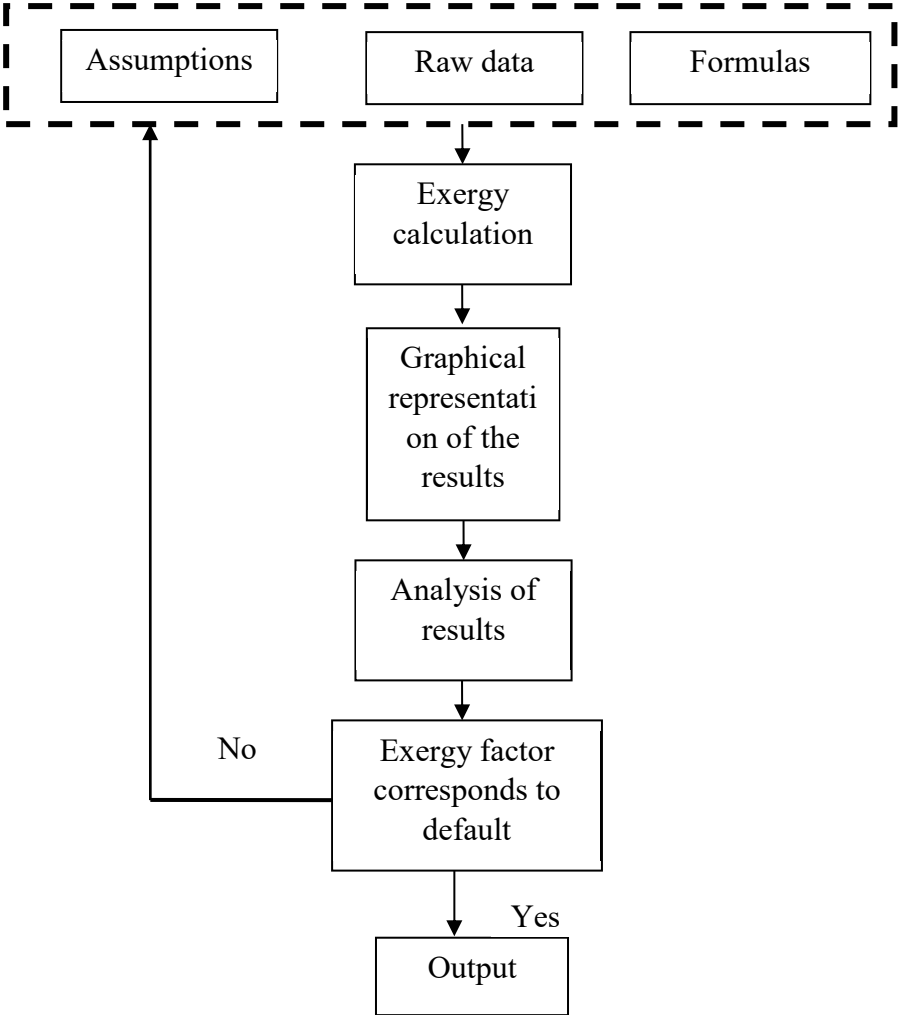
Fig. 1.1. Algorithm of exergy balance model of heat supply system.
