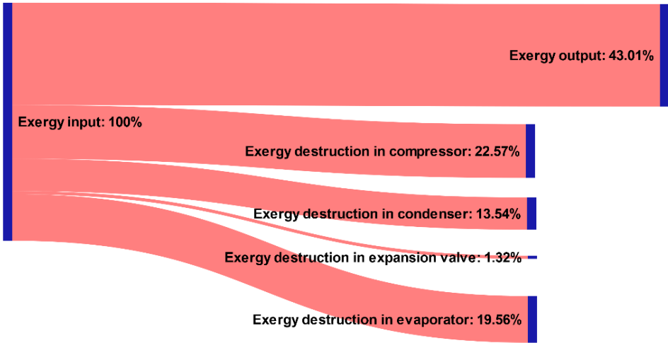
Fig. 2.32. Exergy destruction in two-stage compressor refrigeration system.
