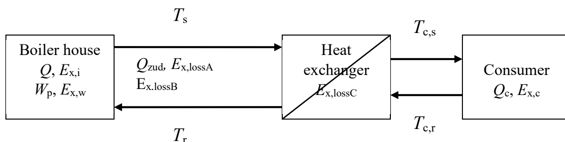
Fig. 2.1. Principal scheme of district heating system.
