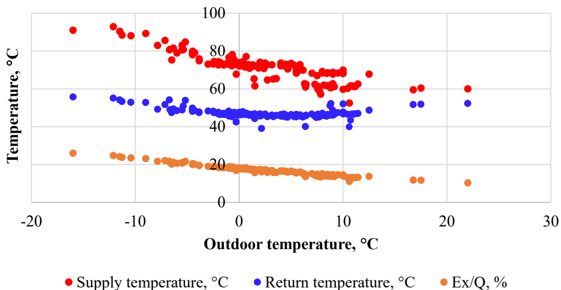
Fig. 2.2. Changes in temperature and exergy factors depending on outdoor temperature.
