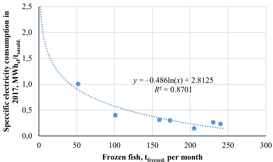
Fig. 2.16. Specific electricity consumption for fish refrigeration.
