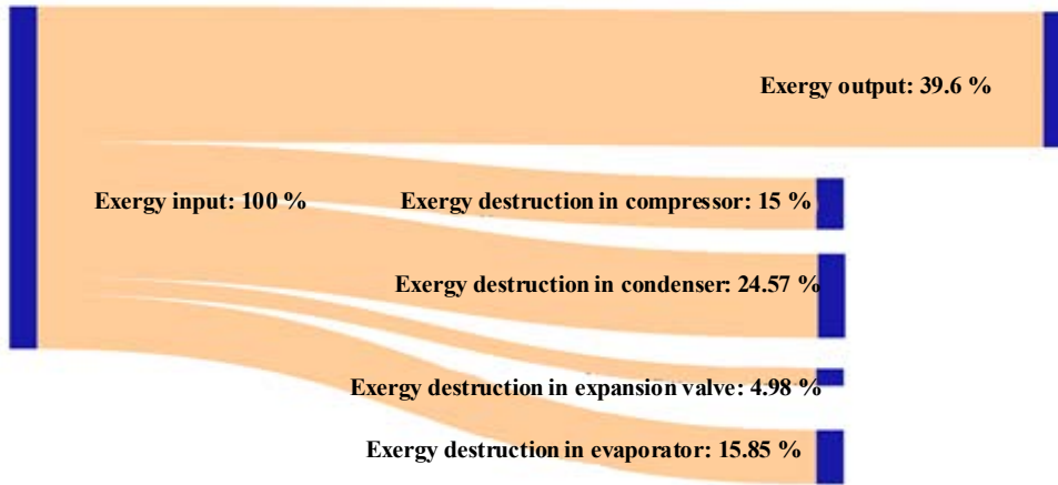
Fig. 2.29. Exergy destruction in single-stage compressor refrigeration system.
