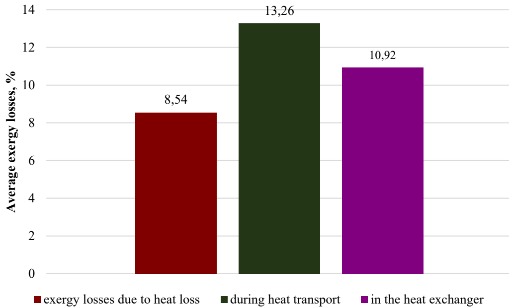
Fig. 2.4. Exergy losses of district heating system.
