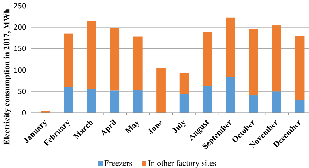
Fig. 2.15. Electricity consumption in fish canning factory.
