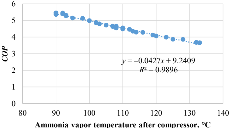
Fig. 2.25. Single-stage compressor COP depending on the ammonia vapor temperature after compressor.
