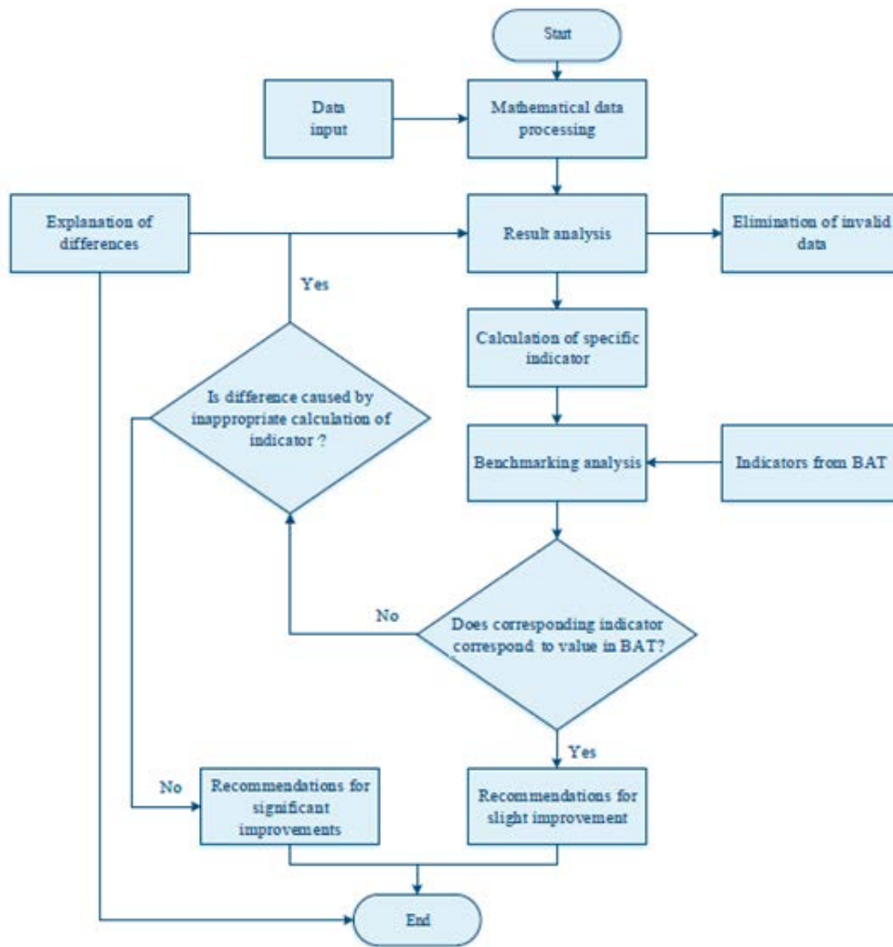
Fig. 2.19. Flow chart of data analysis methodology.
