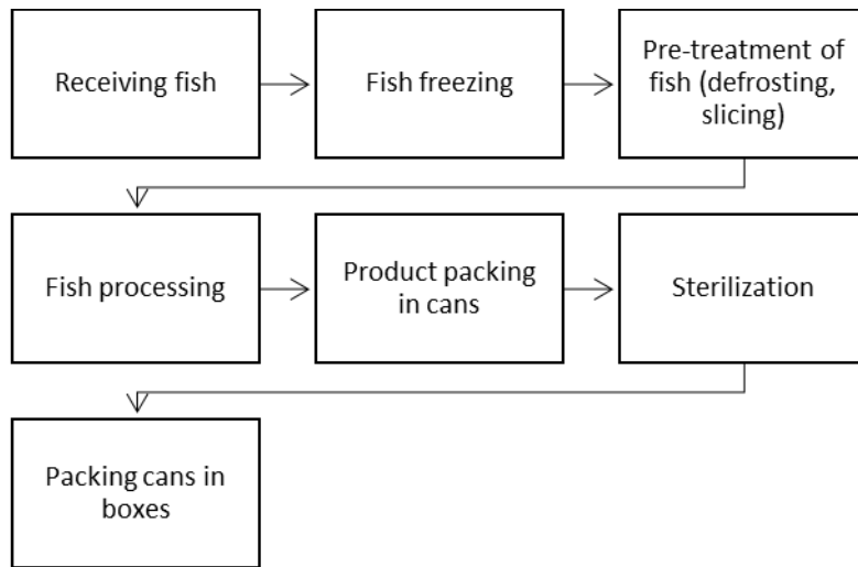
Fig. 2.13. Basic production scheme of canned fish.
