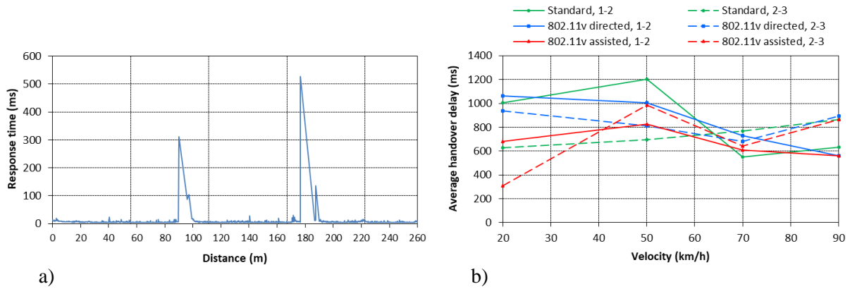
Fig. 16. (a) The response time at 70 km/h and 802.11v network assisted handover; (b) Average handover delay between AP pairs using different handover methods.
