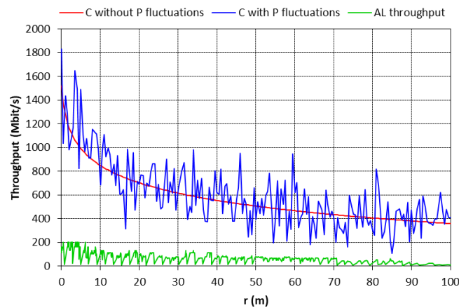
Fig. 20. Theoretically calculated throughput C without and with P fluctuations and experimentally obtained AL throughput depending on the distance to the transmitter.
