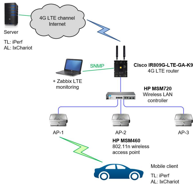
Fig. 9. Network topology of testbed.
