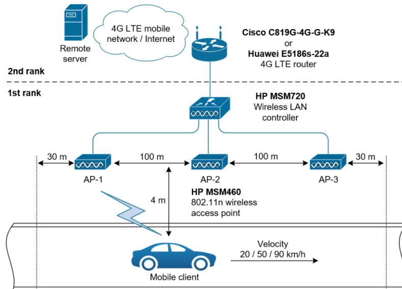
Fig. 3. Network topology of testbed.
