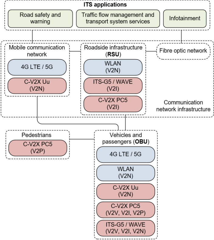
Fig. 2. Combined scheme of ITS communication network technologies.
