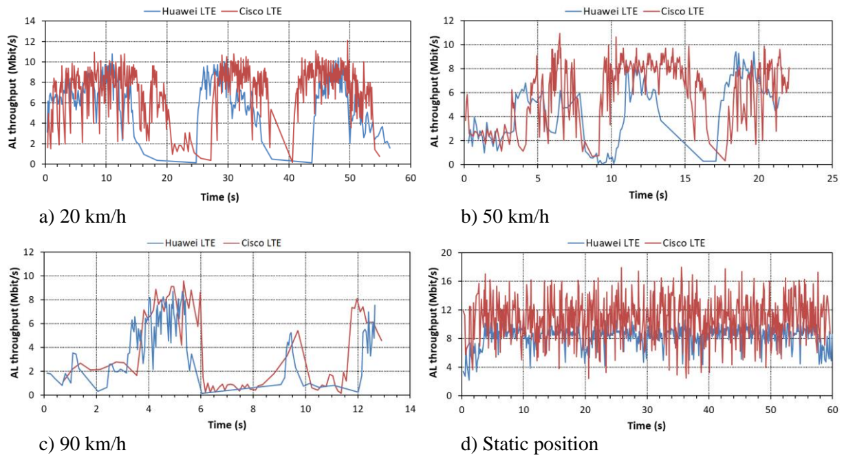
Fig. 4. Comparison of AL throughput using various LTE hardware at various client movement velocities.
