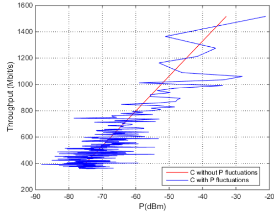
Fig. 19. Theoretically calculated throughput C depending on the received signal power P without and with power fluctuations.
