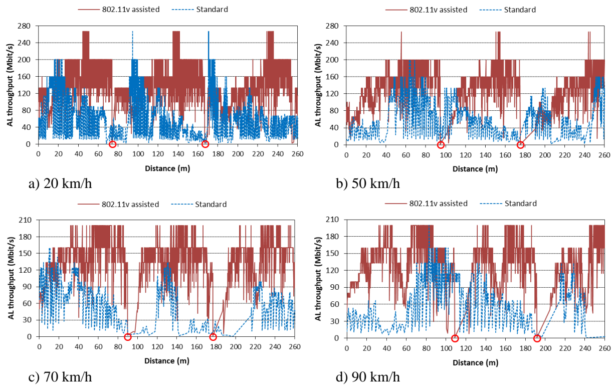
Fig. 14. AL throughput at a velocity of 20 km/h, 50 km/h, 70 km/h, and 90 km/h using 802.11v network assisted and Standard handover methods.
