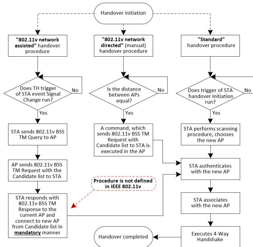
Fig. 12. Summarised scheme of handover algorithms.
