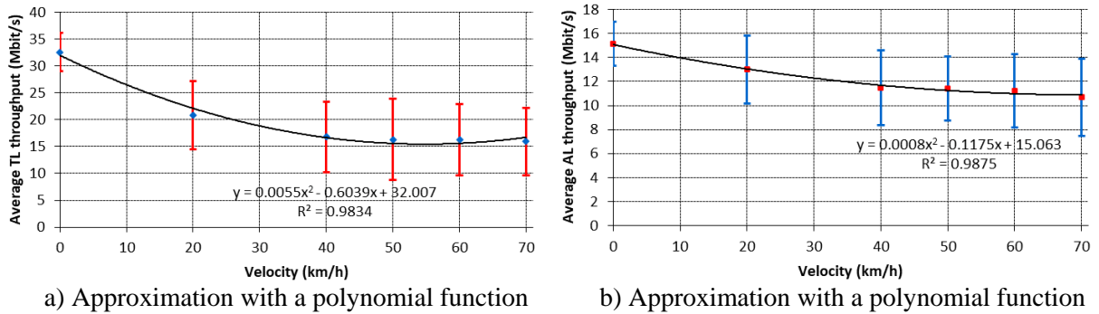
Fig. 11. Approximation of experimental data for the average (a) TL throughput and (b) AL throughput.
