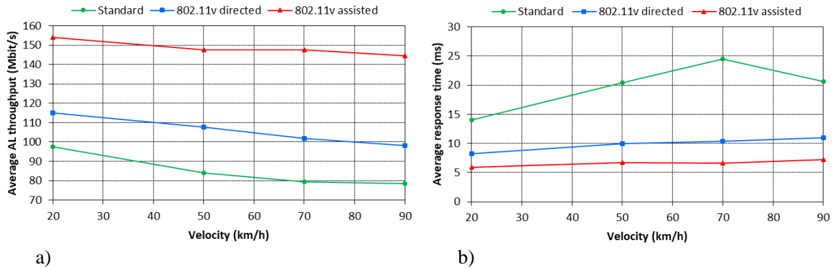
Fig. 15. (a) Average AL throughput; (b) Average response time.
