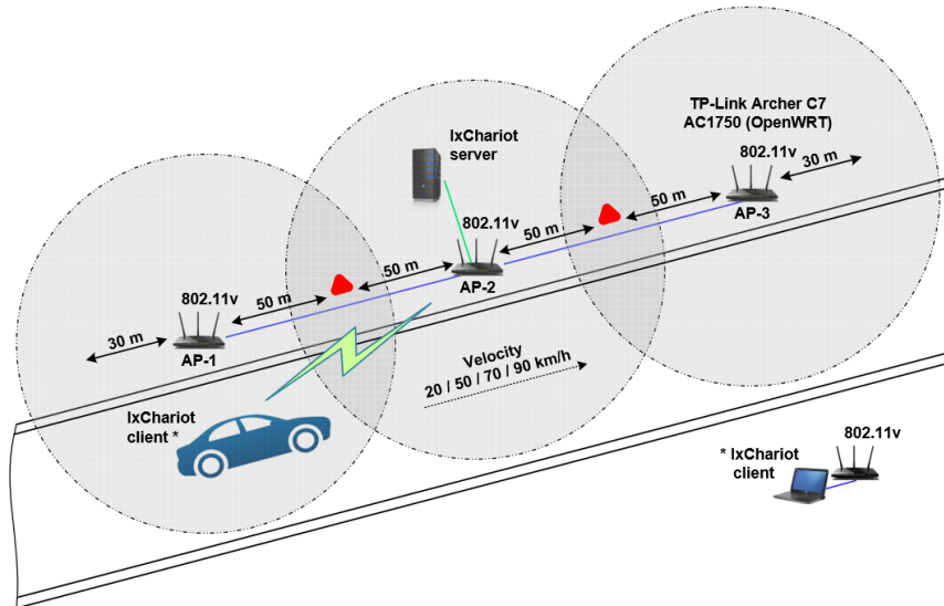
Fig. 13. WLAN IEEE 802.11ac automotive communication network testbed with the introduced modified IEEE 802.11v standard.
