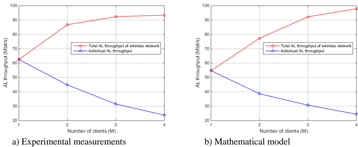
Fig. 6. The determined relationships between the total and individual AL throughput and the number of clients.
