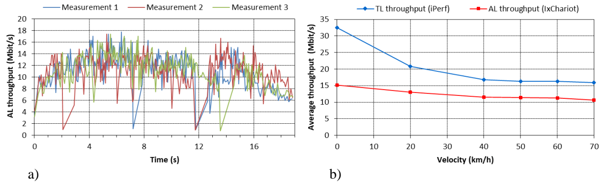
Fig. 10. (a) AL throughput measurement results at vehicle velocity of 50 km/h; (b) The average determined TL throughput and AL throughput of the communication channel depending on the velocity of the vehicle.
