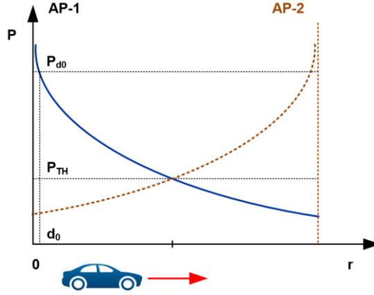
Fig. 17. Alteration of the received signal power parameter P depending on the distance to the transmitter.
