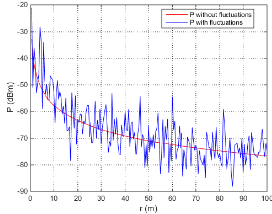
Fig. 18. Theoretically calculated power of the received signal P depending on the distance to the transmitter without and with power fluctuations.
