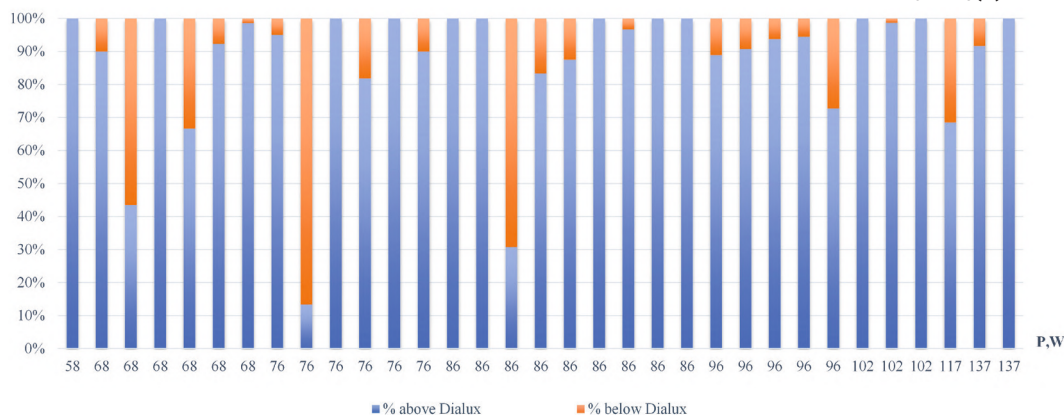
Figure 18. Measured value comparison with Dialux 4.13 obtained result values by luminary power type
