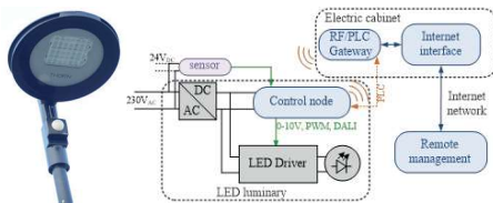
Fig. 1. Developed LITES luminary (right) and LITES system architecture (left)
