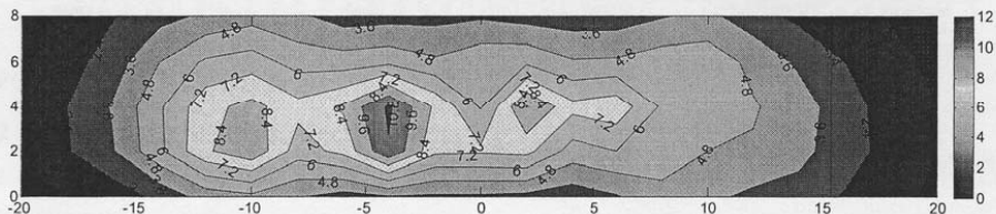
Fig. 7. Measurements for LED luminary at June 30
