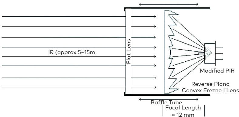
Figure 9. Long-range FoV lens schema
