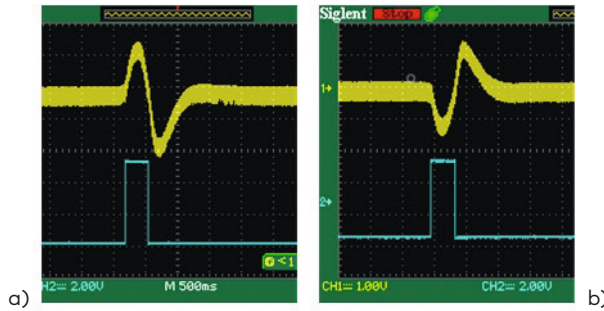
Figure 11. Sensor activation a ~ b, (forward triggering – positive first half cycle) and b ~ a, (reverse triggering – negative first half cycle)
