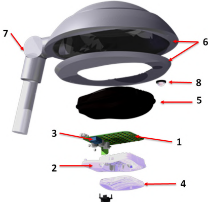
a) LED luminary base elements;
