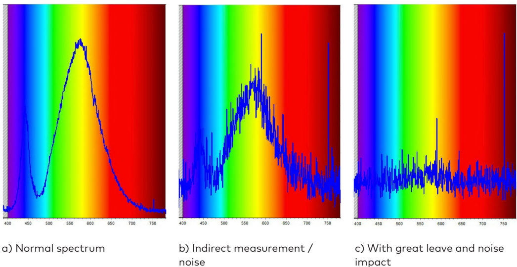
Figure 14. Typical samples of spectrum measurements
