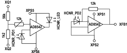
Fig. 5: Optically isolated feedback circuit.
