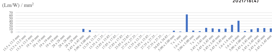
Figure 3. Cree LED manufacturer different LED chip comparison in terms of efficiency (Lm/W per its size in mm 2 ), data obtained at the end of 2020
