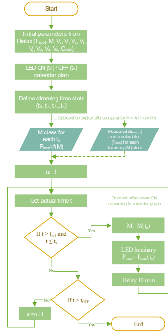
Fig. 11. LED luminaire control algorithm for the scenario without sensor data (standalone regime).
