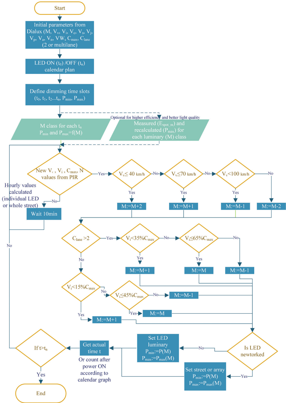
Figure 21. LED luminaire dynamic ME class control algorithm for the proposed sensor system (standalone or networked regime)
