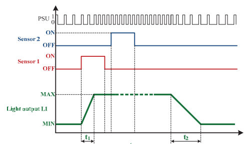
Fig. 2. Example luminary dimming profile in case of sensor triggered lighting control system.
