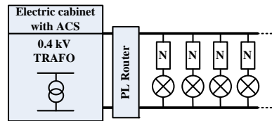
Figure 4. Power Line communication system
