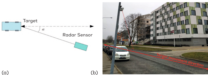
Figure 17. Influence of the radar towards moving object position on the measured speed: (a) schematically (K-LD2); (b) position of the experimental sensor at the installation site
