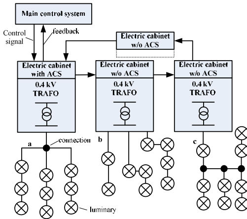
Fig.2. Loop based control system
