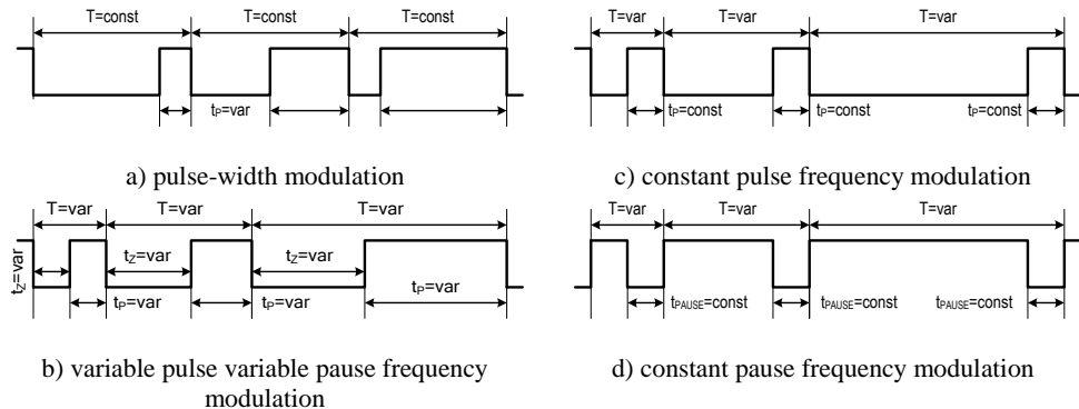
Fig. 3: Pulse modulation methods for LED dimmers.
