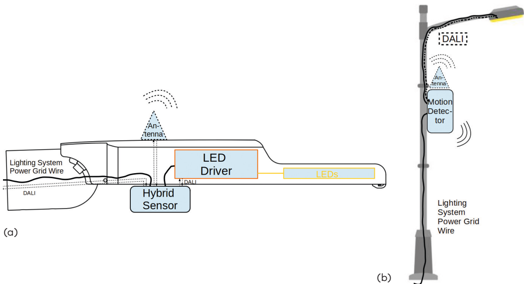
Figure 18. Two reasonable sensor installation possibilities: (a) on a street lamp itself; (b) on a street light pole
