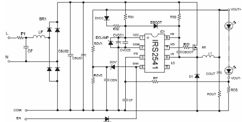
Fig.2. Electrical circuit of IRS2541 LED Driver.
