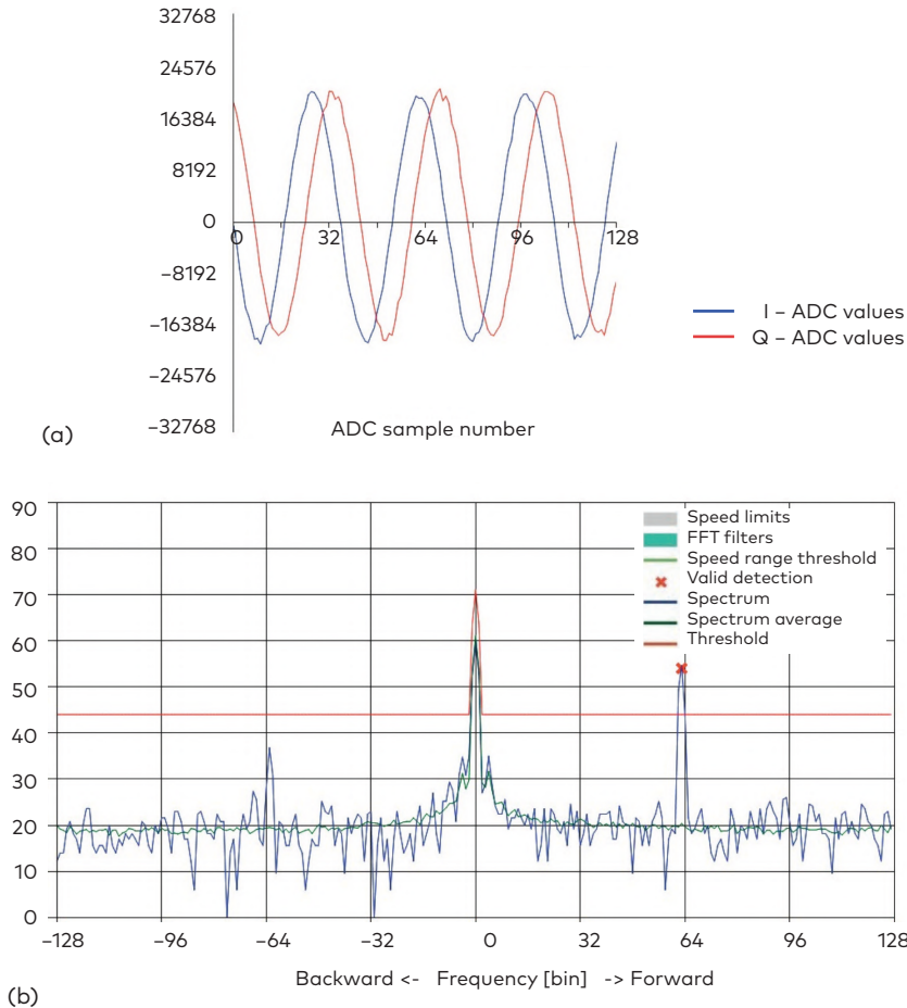
Figure 16. Radar transceiver signals: (a) I/Q signals; (b) complex FFT derived from I/Q signals (K-LD2)
