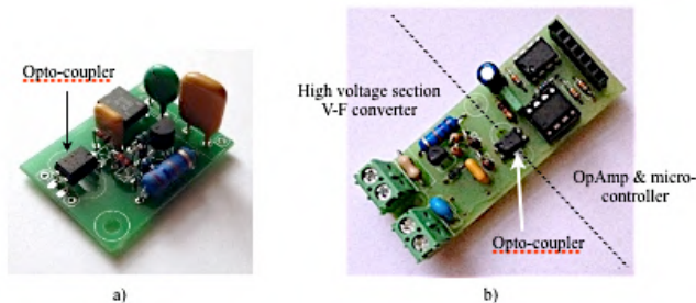
Fig.4. Energy metering devices prototypes: a) simple voltage-frequency converter module, b) with integrated voltage-frequency converter, current transformer operational amplifier and ATtiny85 micro-controller
