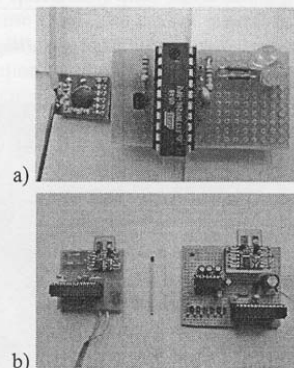
Fig. 8. Laboratory experimental transceiver prototypes with a) RFM12B with ATtiny861V, b) MRF24J40MA with ATmega88PA.
