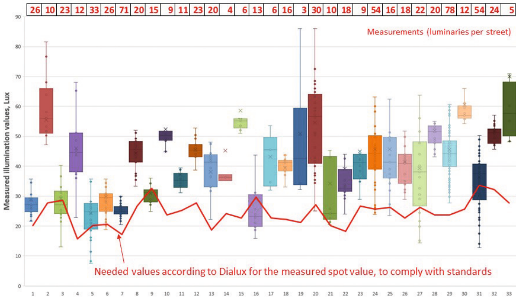
Figure 17. The measured illumination value distribution per street and needed minimums, according to Dialux
