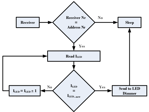
Fig. 2.12. Simplified control algorithm.
