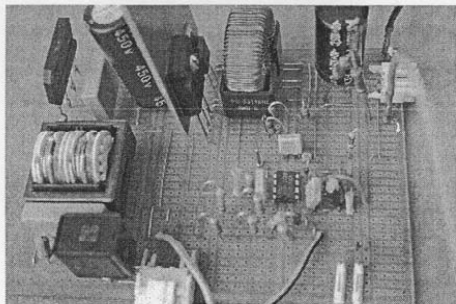
Fig. 6. Laboratory experimental prototype of IRS2541 LED Driver
