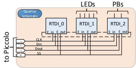
Fig. 5. Quartus block scheme for global RTDI
