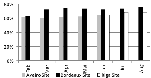
Fig. 13. Energy savings in LITES project Pilot Sites.
