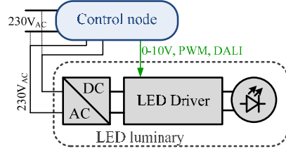
Fig. 2. Architecture with control node.
