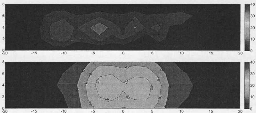
Fig. 10. General comparison in scale of 40 lx. Top – LED, bottom – NaHPS
