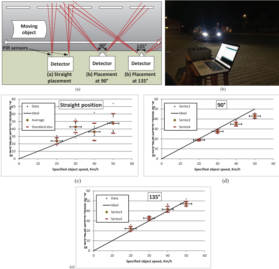
Fig. 3. Tests on the considered PIR detector prototype: (a) block diagram; (b) field tests; (c), (d) and (e) summary of the test results.
