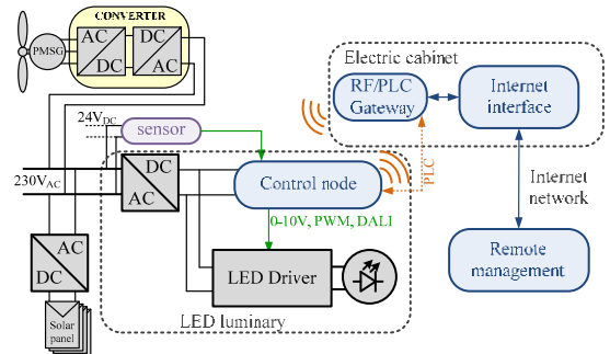
Fig. 6. Architecture with AC grid connected renewables.
