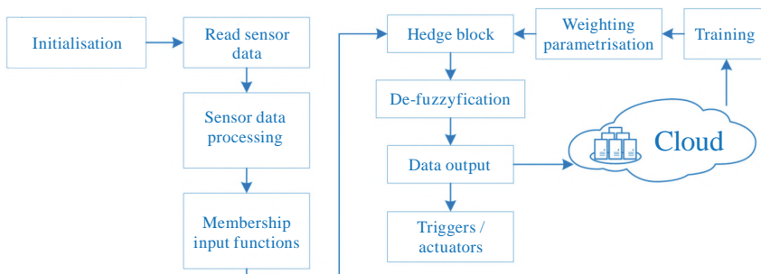
Figure 6. Fuzzy logic block diagram of agent and cloud interaction
