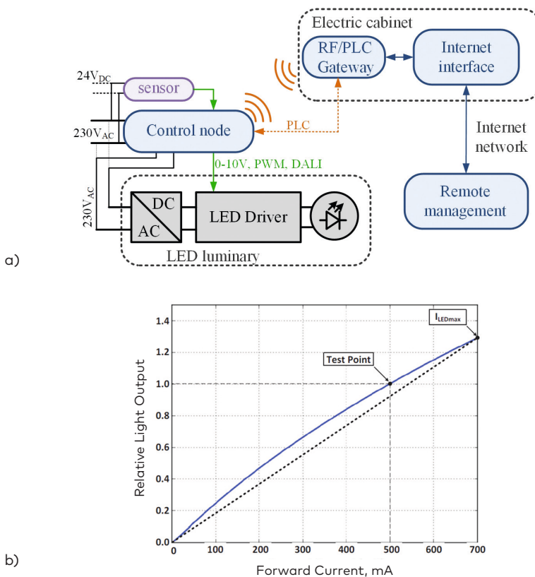
Figure 9. A sample of smart lighting LED luminary (a), and the relation between LED current and light output (b)
