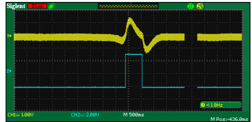
Fig.6. Slower movement can be indicated by overshoot or undershoot of the waveform.
