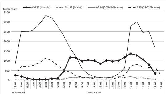
Fig.5. Traffic intensity measurement data obtained from internet databases.
