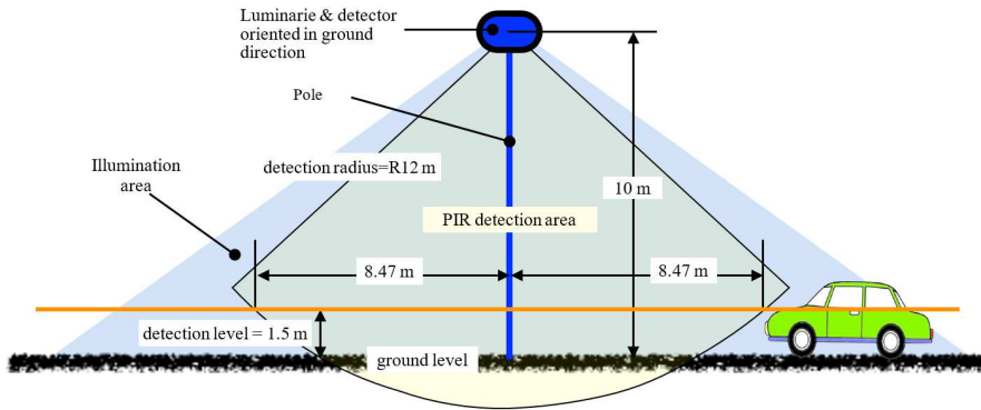
Fig. 4. Luminaire and detector position on the mast and corresponding dimensions, illumination and detection areas.
