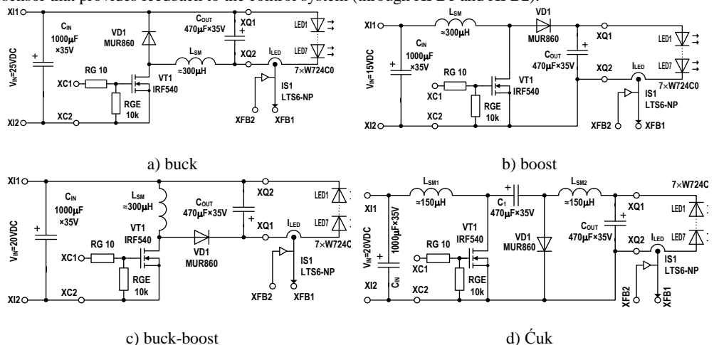
Fig. 2: Dimming DC/DC converters for light regulation with LEDs.
