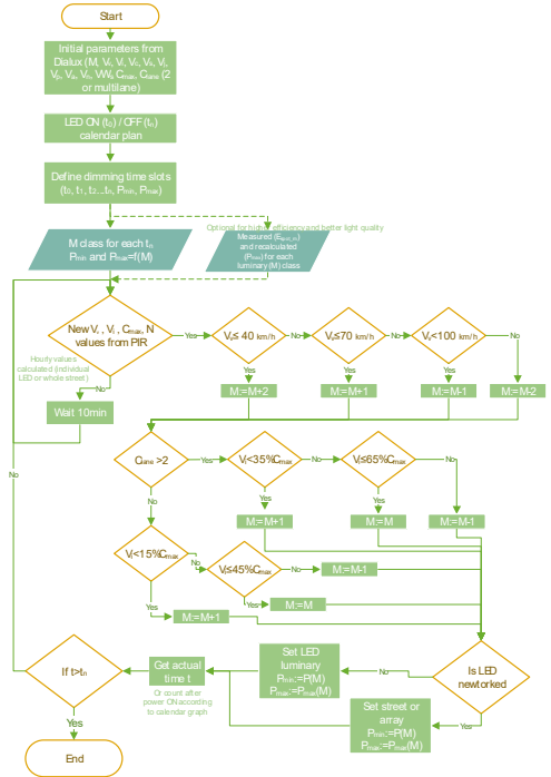
Fig. 12. LED luminaire adaptive control algorithm for the scenario with smart sensor data (standalone or networked regime).
