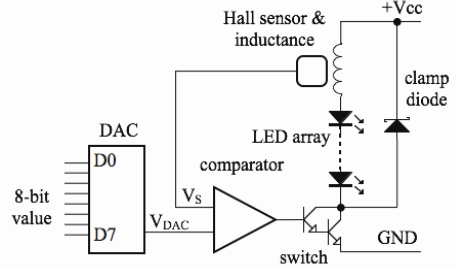
Fig.5. Schematics of LED driver circuit
