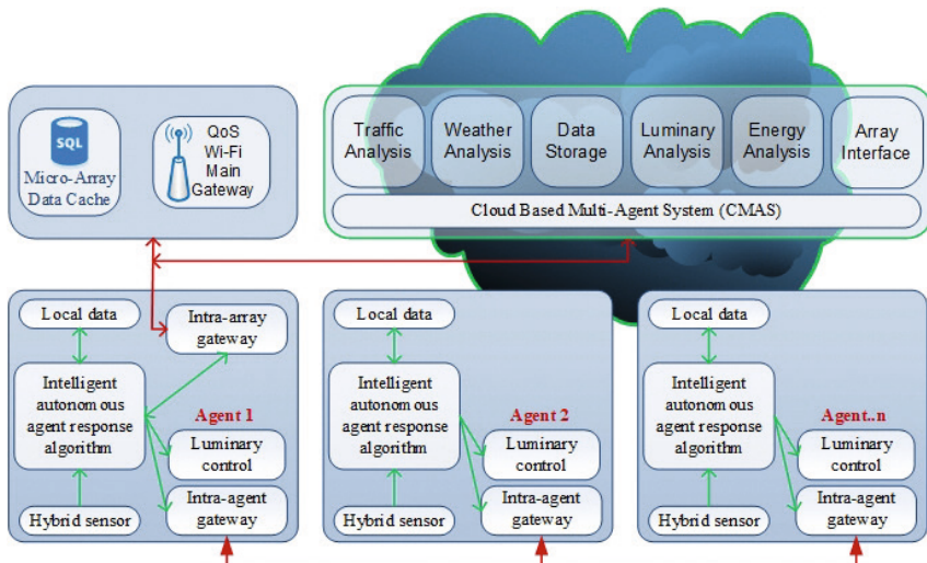
Figure 7. Cloud-based multi-agent system model
