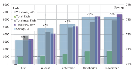
Fig. 4. Energy consumption at Riga Pilot Site
