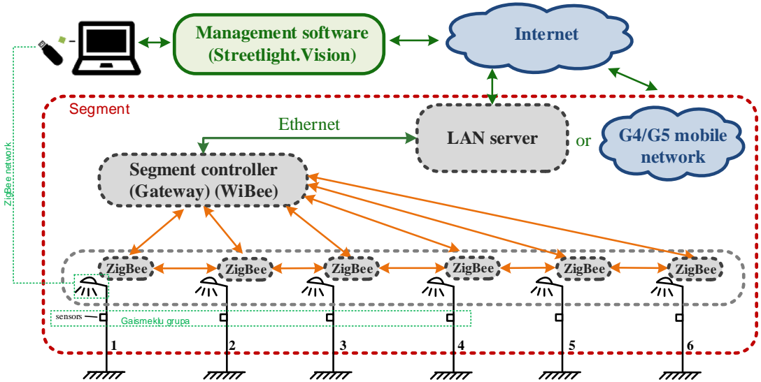
Fig. 4.3. Structural diagram of created smart lighting system.
