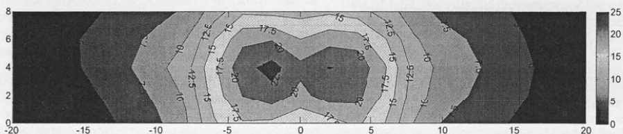
Fig. 8. Measurements for NaHPS luminary at June 16
