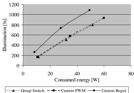
Fig. 5. Efficiency of dimming control methods
