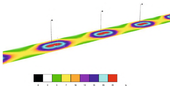
a) Dialux simulation model (results of 150W HPS)
