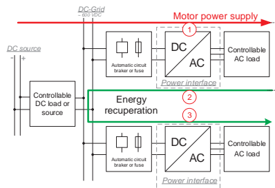
Fig. 3. DC-based power architecture (1-3 = AC/DC conversion stages).
