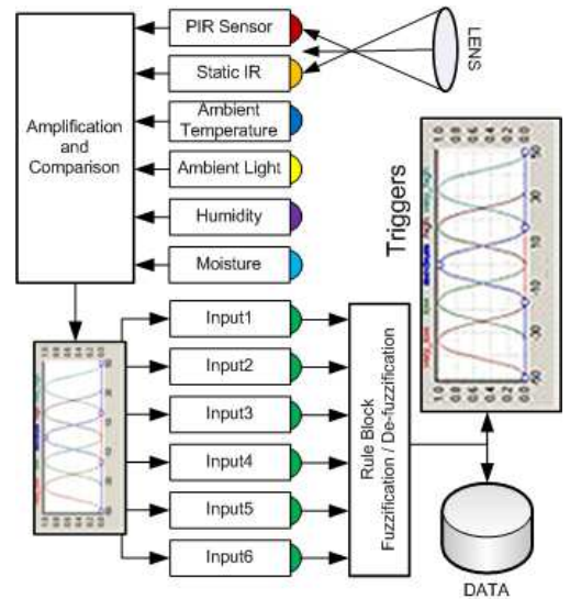
Fig.2. Current fuzzy logic system model.
