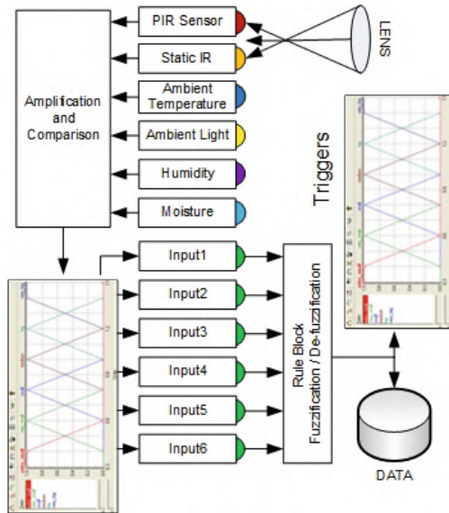
Figure 3. Original fuzzy logic system model. Recent model addition includes Radar module
