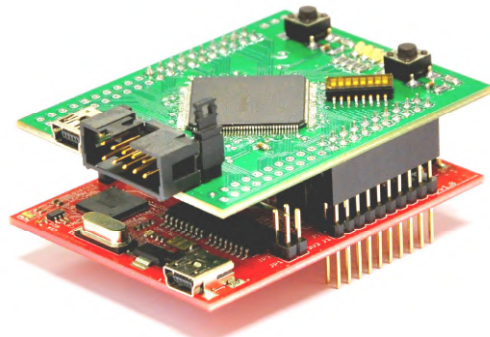
Fig. 2. Stacked connection of FPGA and Piccolo LaunchPad boards.
