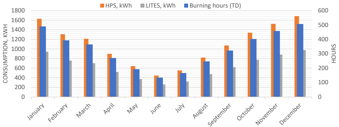
Fig. 4.9. Analytically calculated electrical energy consumption for high pressure vapour (HPS) and smart LED luminary cases.
