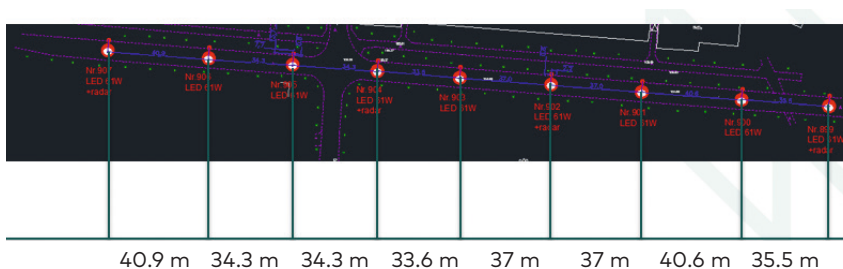
Figure 6. Sample of AutoCAD format (*.dwg file) topographical layout for street lighting with various pole distances
