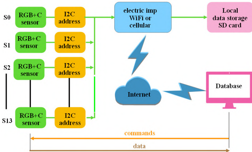
Fig. 6. Data receiving and commands sending scheme
