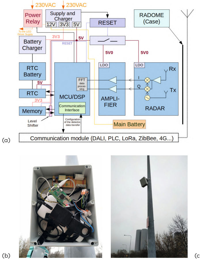
Figure 19. Radar sensor for experimental verification: (a) block schematics; (b) and (c) practical realisation
