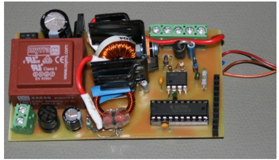
b) dimmer with integrated control module.
