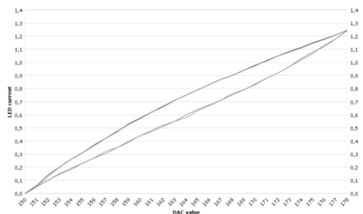
Fig.7. LED current vs DAC output value of developed Hall Sensor
