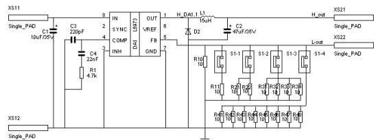
a) electrical diagram
