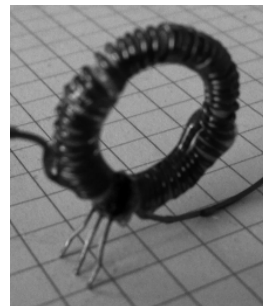
Fig.6. Inductor and Hall Effect sensor
