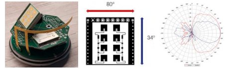
a) Transceiver itself b) antenna beam aperture.
