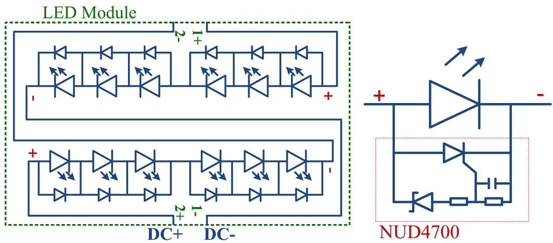
a) LED PCB schematic of one module; b) active shunt.
