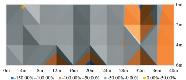
Figure 11. Incukalns city street comparison in 2012: a – street profile; b – comparative difference (%) between the measured and modelled street profile values
