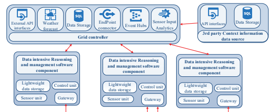
Fig.4. Basic software architecture for context integration.
