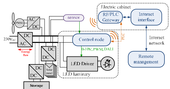
Fig. 7. Architecture with DC grid connected renewables.
