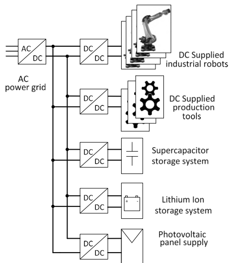
Fig. 2. Example of industrial DC microgrid structure
