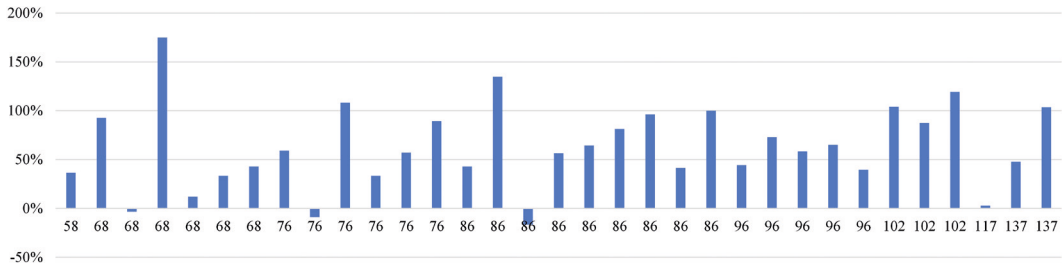
Figure 19. Light difference between Dialux and measured values by LED luminaire power
