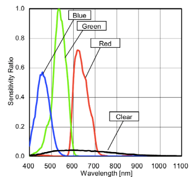
Fig. 3. Sensor sensitivity-wavelength relationship graph
