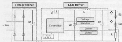
Fig. 5. Functional diagram of LED controlling with IRS2541
