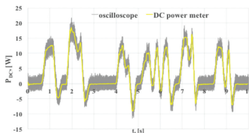
Fig. 7. Noise impact –Oscilloscope v.s. Bi-directional AC/DC power / energy flow meter (20 ms energy sampling rate).
