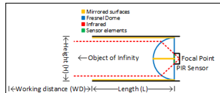
Fig. 6. Lens adaptor long and short-range configuration.
