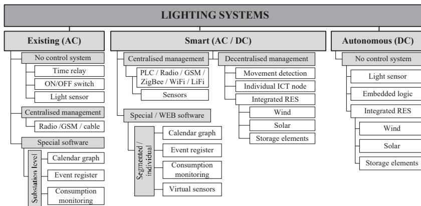
Fig.3. Classification of LED based lighting system architectures.
