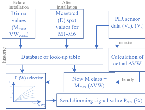
Fig. 8. Simplified control algorithm block diagram of a single luminary.
