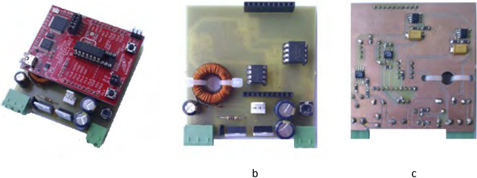
Fig. 6: Laboratory assembly: a) LED dimmer controlled by LaunchPAD; b) power board TOP; c) power board BOTTOM
