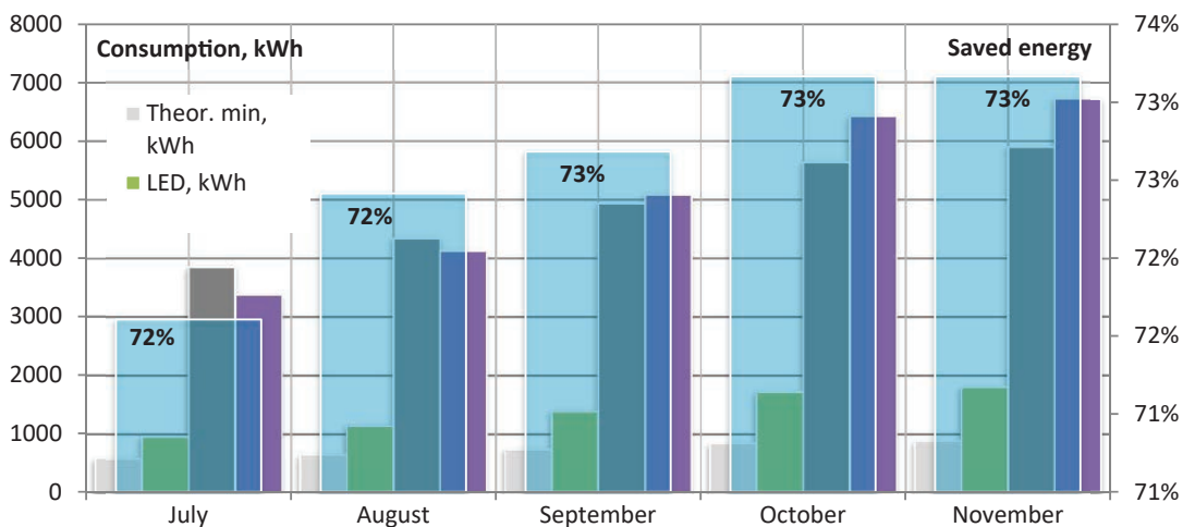
Fig. 4.12. Real energy consumption of smart lighting system at Kipsala Pilot Site.
