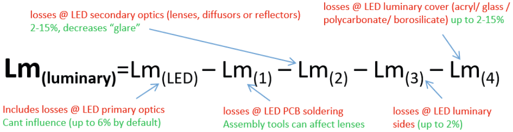
Figure 1. Typical places of total luminary lumen losses in LED luminary manufacturing process
