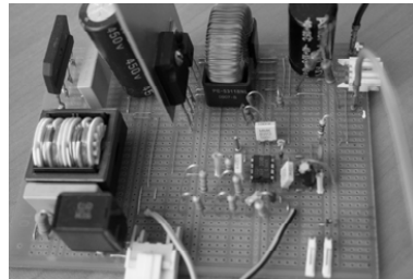
Fig.3. Laboratory experimental prototype for IRS2541 LED Driver.
