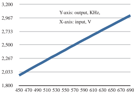
Fig.4. Voltage to frequency conversion curve
