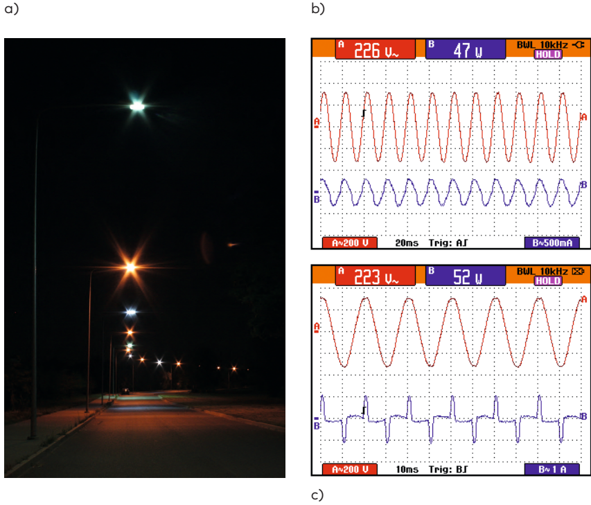
Figure 10. Results of measurements performed in 2009: a – picture of dry road PilotSite in Riga; b – AC voltage and current waveform for Cobrahead 48.7W luminary; c – AC voltage and current waveform for Diodella 52W luminary
