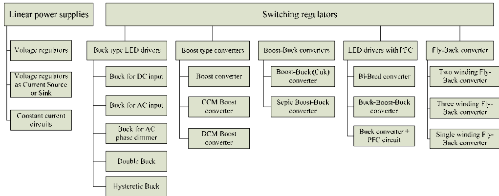
Fig. 1. Power supply topologies suitable for LED driving.
