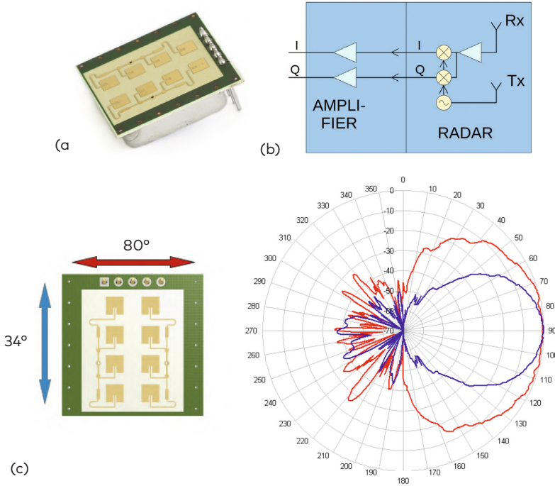
Figure 15. Selected transceiver for radar sensor: (a) appearance; (b) block diagram; (c) antenna system diagram (K-LC2)
