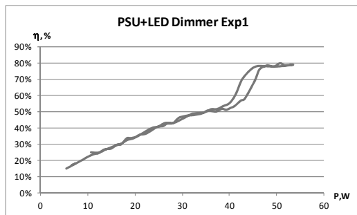
Fig.12. Efficiency of LED power supply with Dimmer
