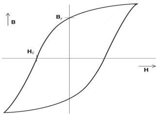
Fig.5. Typical ferromagnetic magnetisation B-H curve
