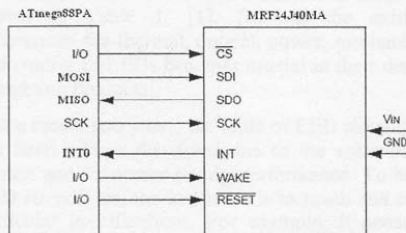
Fig. 10. Microcontroller ATmega88PA to MRF24J40MA interface
