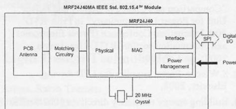
Fig. 11. MRF24J40MA block diagram
