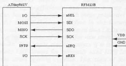
Fig. 9. Microcontroller ATtiny861V to RFM12B interface
