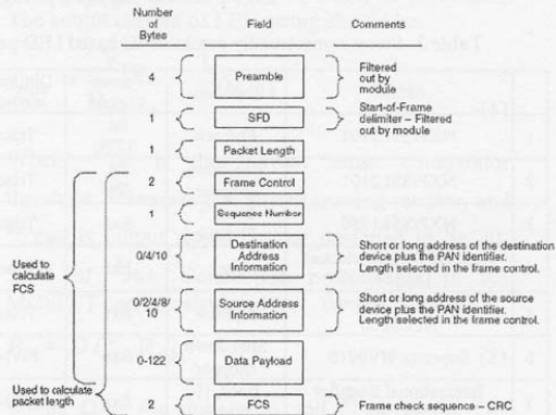
Fig. 7. IEEE 802.15.4 compliant packet format
