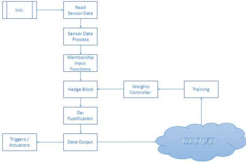
Fig.8. Decentralized Controller Flow Chart.
