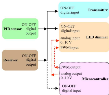
Fig. 5. System functional diagram.
