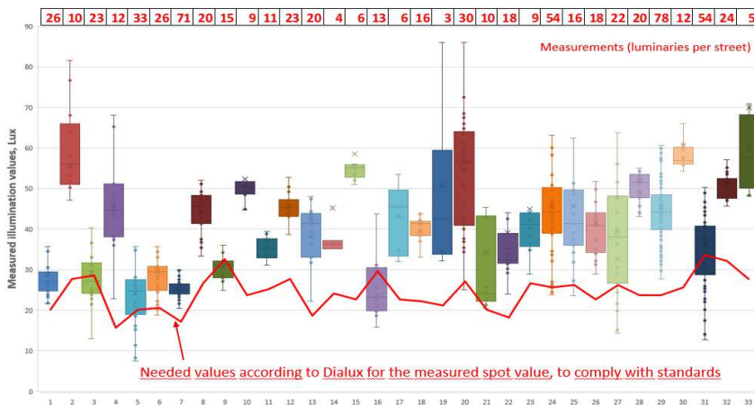
Fig. 3. Measured illumination vale distribution per street and needed minimums, according to Dialux.
