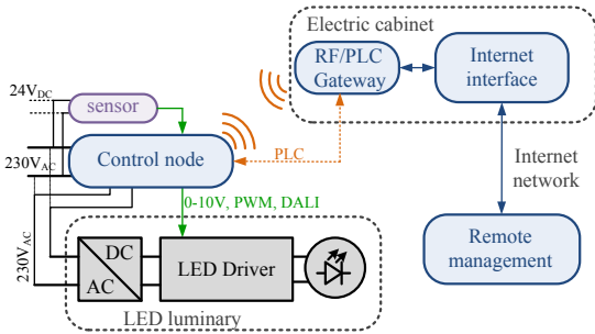
Fig. 4. Architecture with control node and movement detection sensor.
