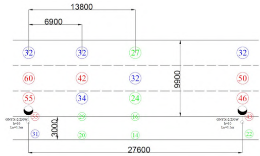
Fig. 4. Practical luminous (Lux) value measurements on site.
