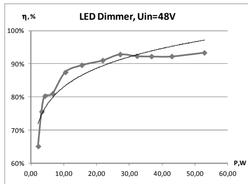
Fig.13. Efficiency of LED Dimmer
