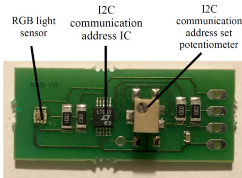
Fig. 2. Individual RGB light sensor
