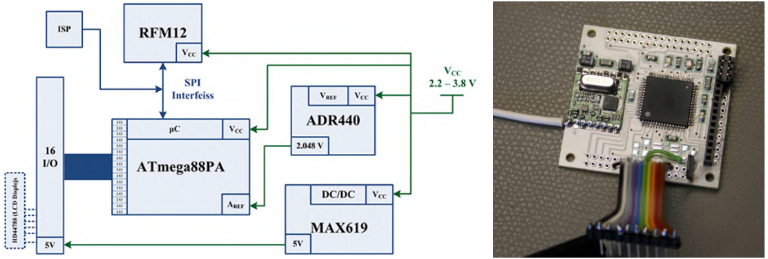
a) communication module block diagram;
