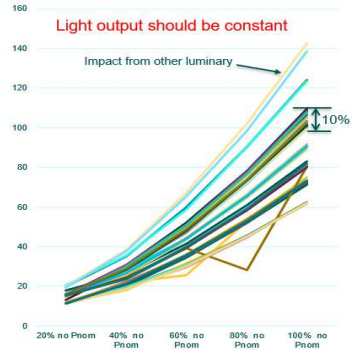
Fig. 1. Graphical relation of active power consumption and dimming step value.
