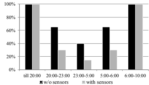
Fig. 10. Minimal light output values for dimming profiles.
