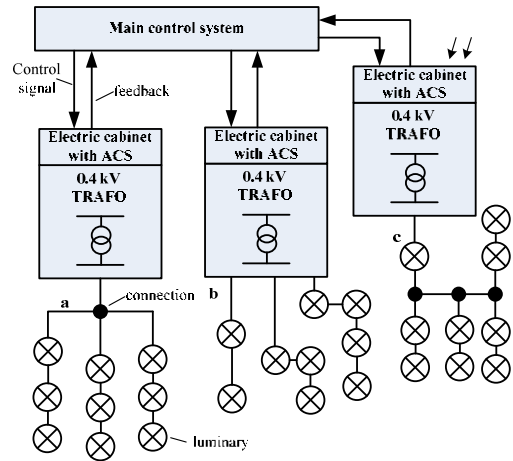
Fig.3. Automated control system
