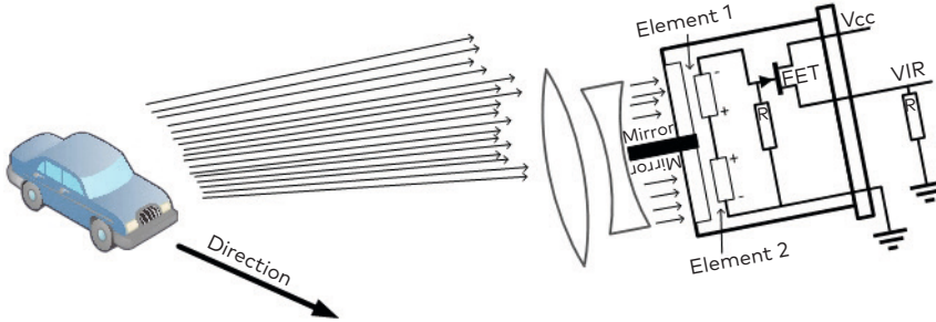
Figure 8. Long-range PIR methodology
