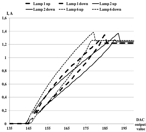
Fig.8. DAC output value of various LED Lamps
