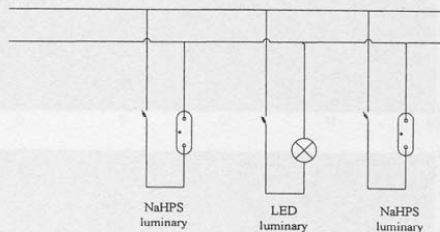
Fig. 5. Connection of luminaries
