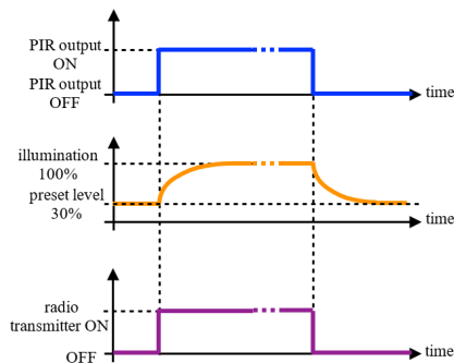
Fig. 6. Process diagrams.
