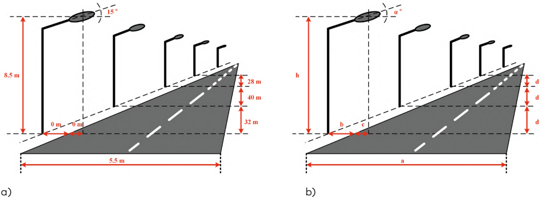
Figure 5. The necessary geometrical input data for Dialux light distribution calculations
