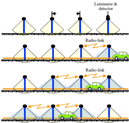
Fig. 2. Luminaire and detector position on the street or the walkway and "wave" operation.
