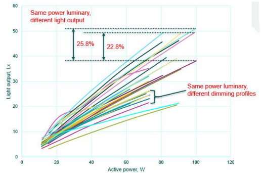
Fig. 2. Graphical relation of power consumption and measured light output values.
