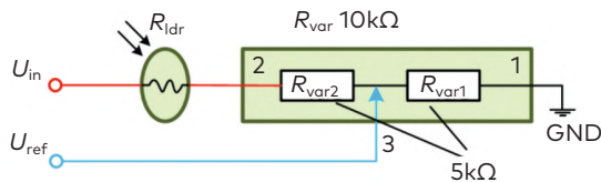
Figure 5. LDR /VAR potential divider configuration for ambience control
