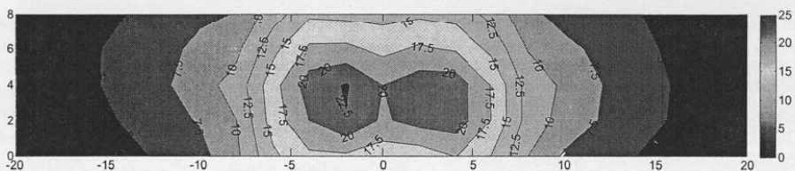
Fig. 9. Measurements for NaHPS luminary at June 30
