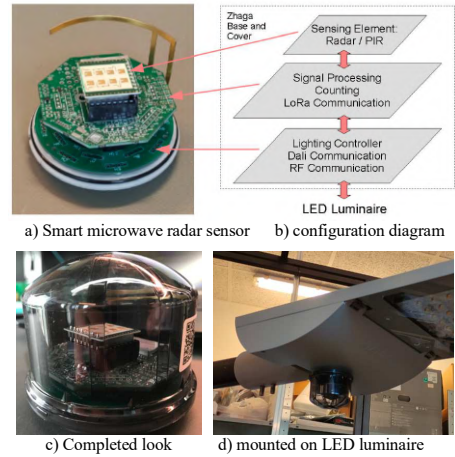
Fig. 4. Configuration of intelligent movement sensor
