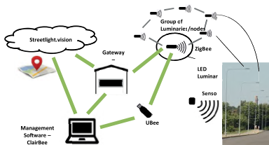
Fig. 2. LITES technology communication architecture
