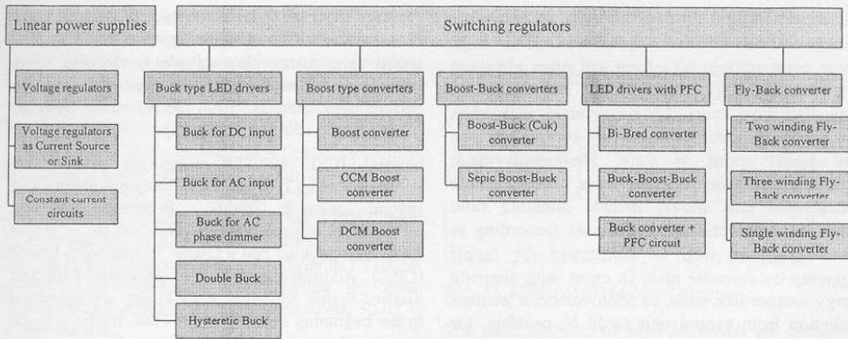
Fig. 4. Power supply topologies suitable for LED driving
