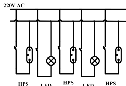
Figure 3. On-site luminary layout..
