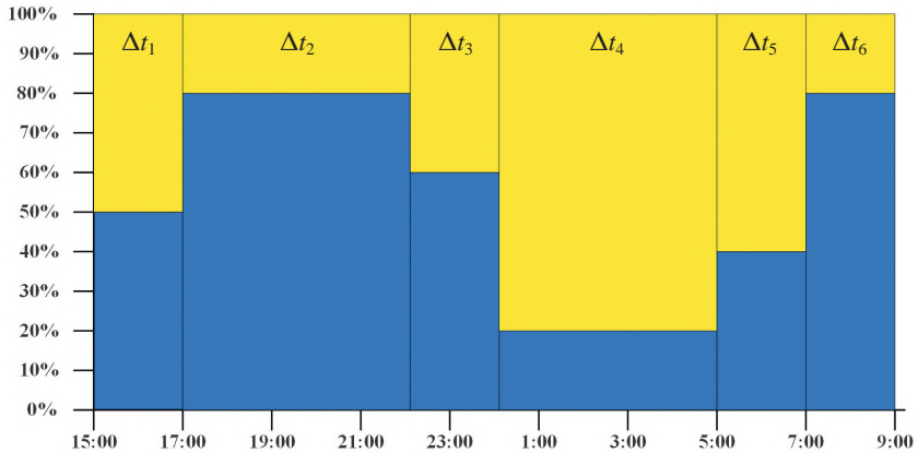
Figure 4. LED luminary nighttime intervals and programmed power output minimums/maximums for the movement sensor triggering signal control
