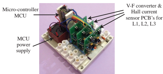
Fig.3. AC 3-phase bidirectional energy consumption measurement module
