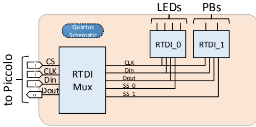
Fig. 4. Quartus block scheme for multiplexed RTDI.
