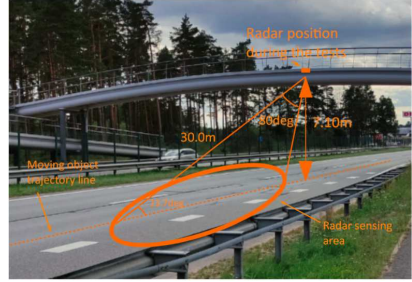
Fig. 10. In-situ experiments with radar module, sensing area, and angles.
