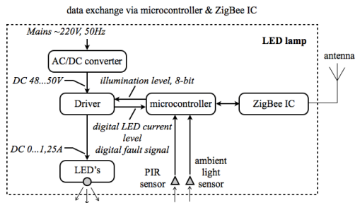
Fig.11. Internet and ZigBee PAN control network
