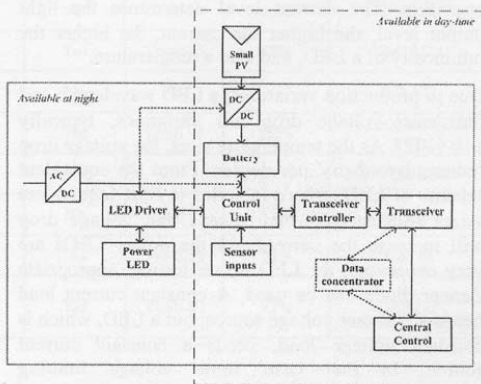
Fig. 3. Basic concept of intelligent LED luminary
