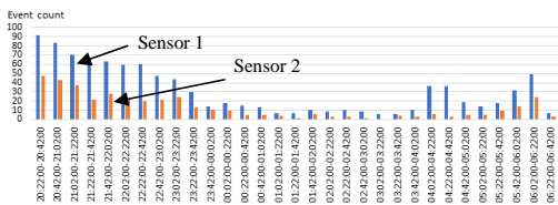
Fig. 6. Sensor event count each 20 min during 03.04.2019.-04.04.2019.
