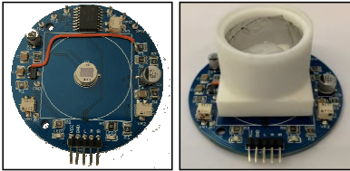
a) PIR Sensor mainboard. b) prototype with lens adaptor.
