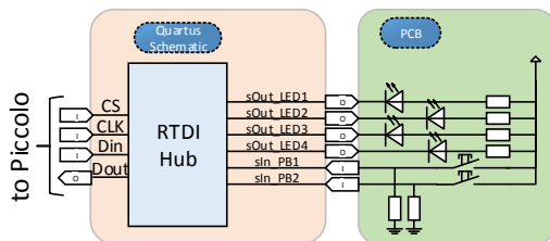
Fig. 3. Quartus block scheme for central RTDI.
