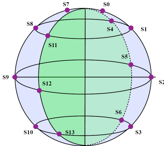
Fig. 5. Sensors' positions on the spherical surface
