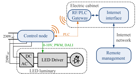
Fig. 3. Architecture with control node with communication circuit.
