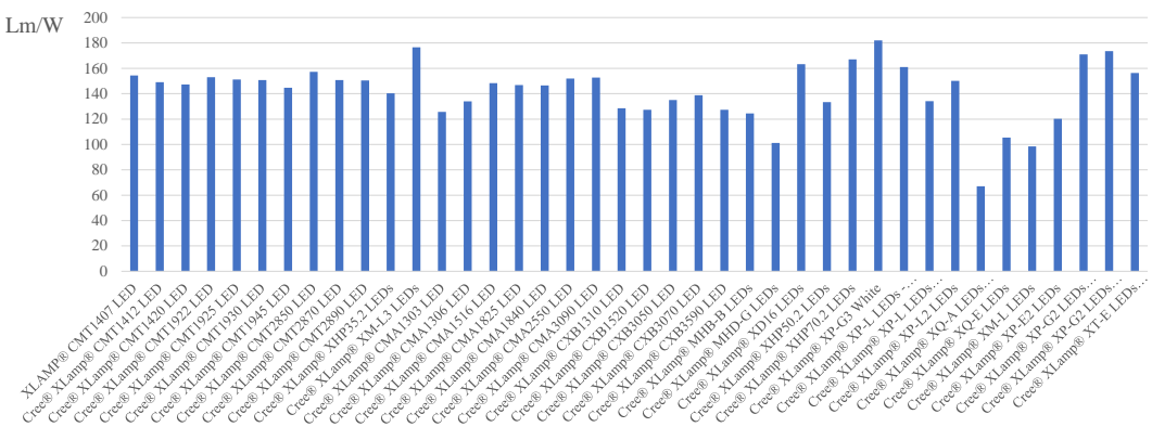
Figure 2. Cree LED manufacturer different LED chip comparison in terms of efficiency (Lm/W), date obtained at the end of 2020
