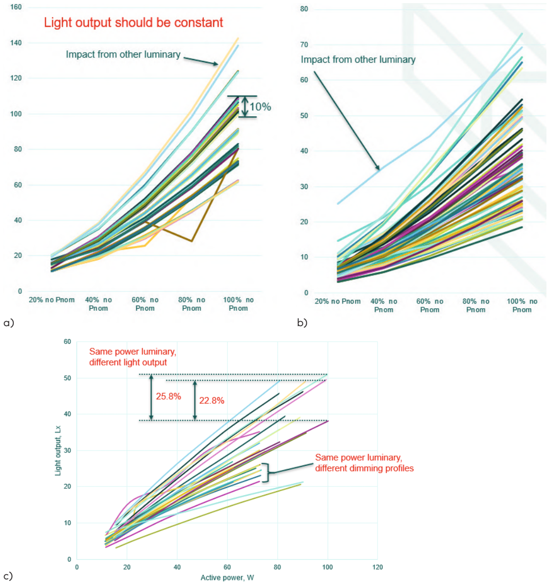
Figure 16. Graphical relation of power consumption, dimming value and measured light output values
