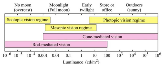
Fig. 1. Approximal vision and receptor regimes.
