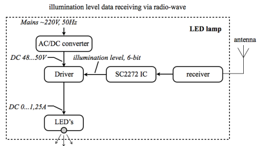
Fig.9. Radio wave link as control signal
