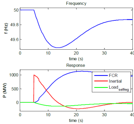
Fig. 1.1. Frequency, inertial, and FCR response to a generator outage [5].
