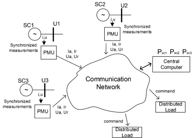
Fig. 2.2. Potential measurement/command arrangement for the proposed LS scheme.
