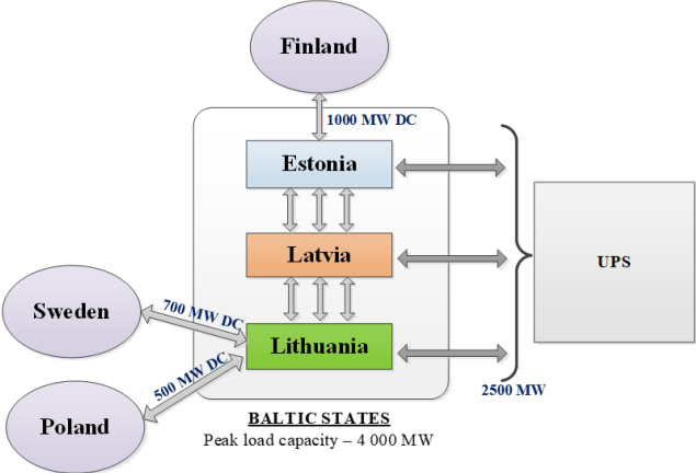
Fig. 1.5. Schematic power system interconnection of the Baltic states.
