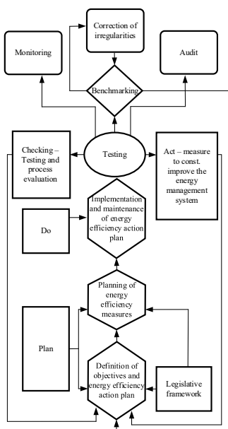
Fig. 2.4. Energy management framework for the agricultural sector at the company level.
